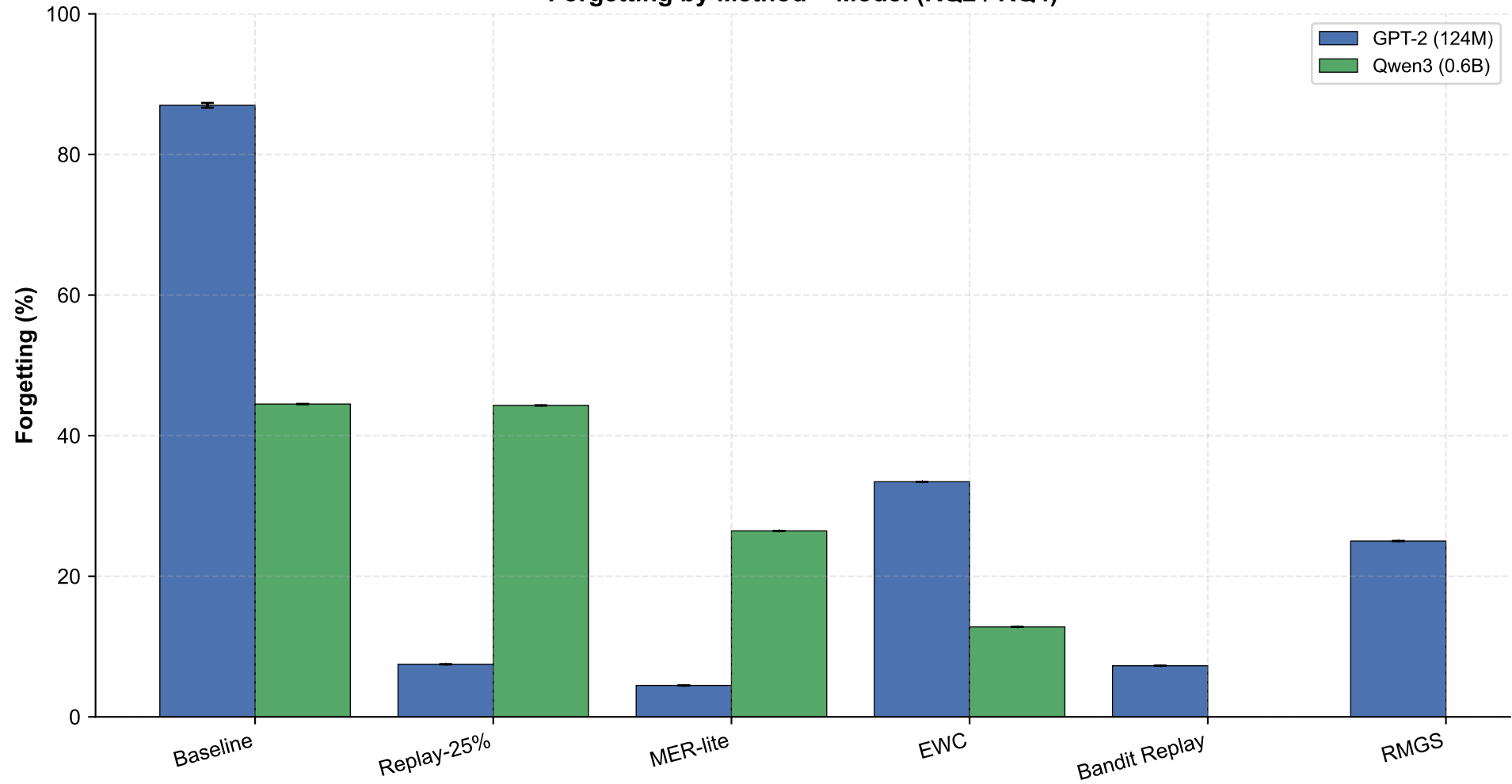
Forgetting by Method × Model (RQ2 / RQ4)
