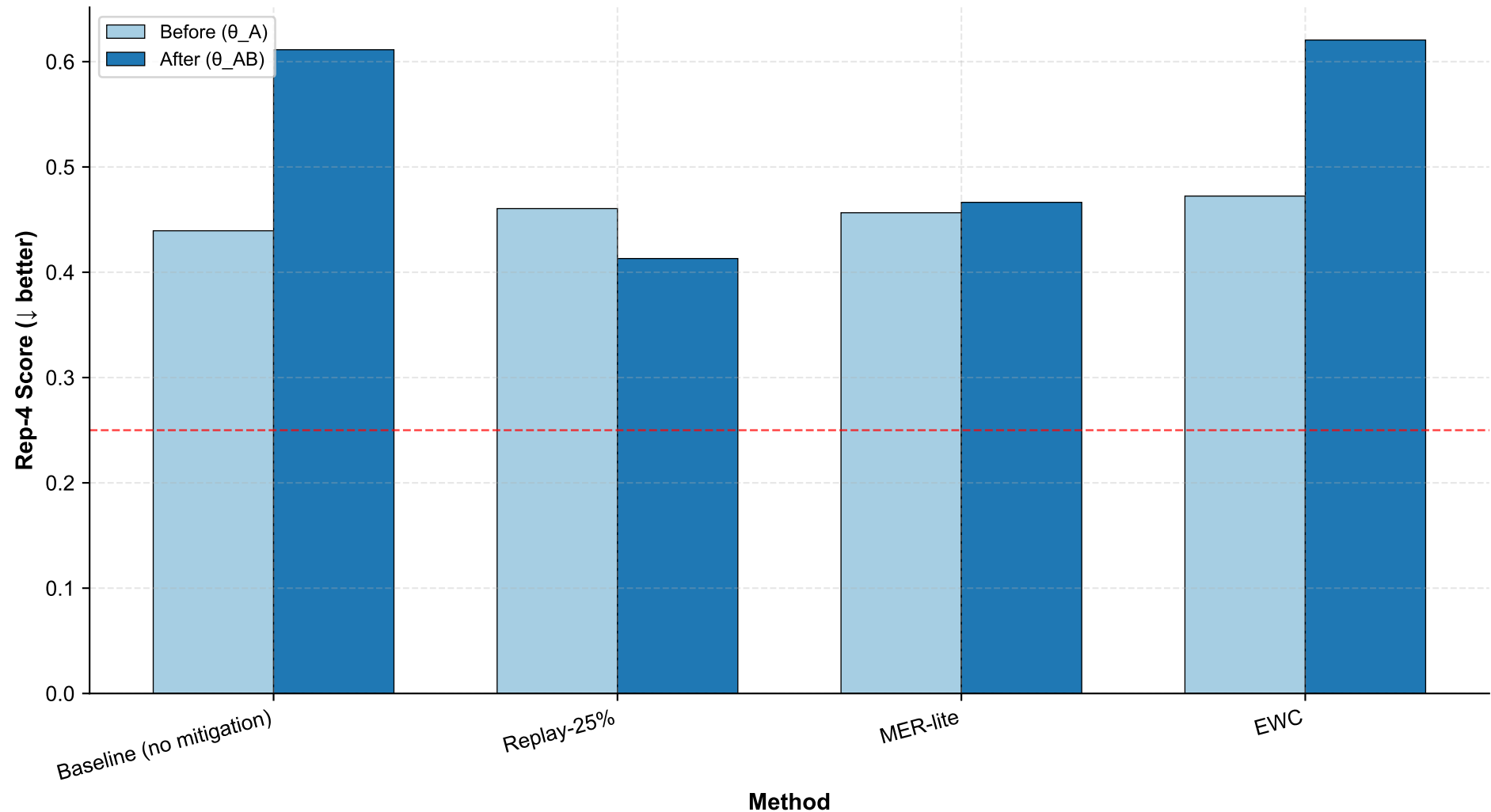
Repetition (4-gram) Before vs After Domain B Training (wikitext-103 \rightarrow arxiv_abstracts)
