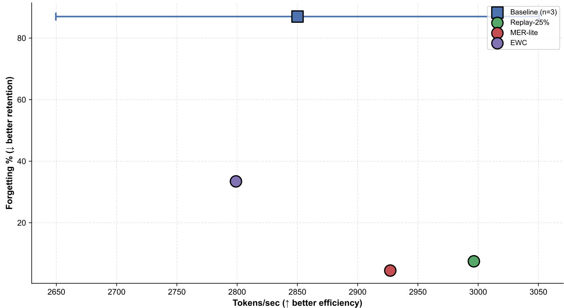
Compute Efficiency vs Retention Tradeoff (wikitext-103 \rightarrow arxiv_abstracts)
