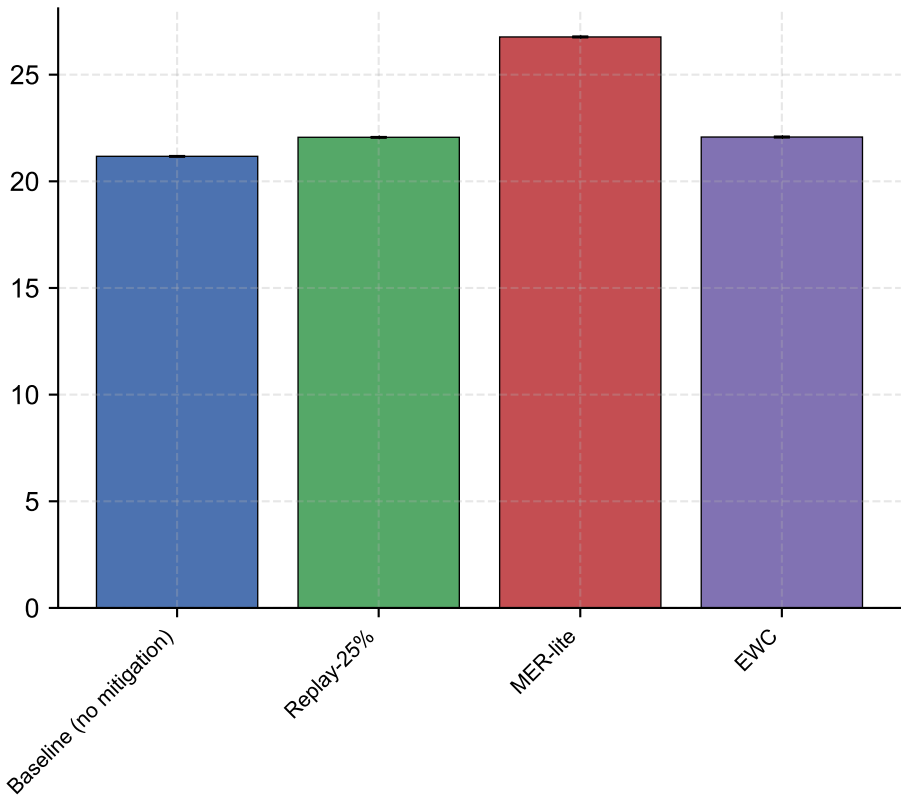
PPL on Domain B (↓ better adaptation)
