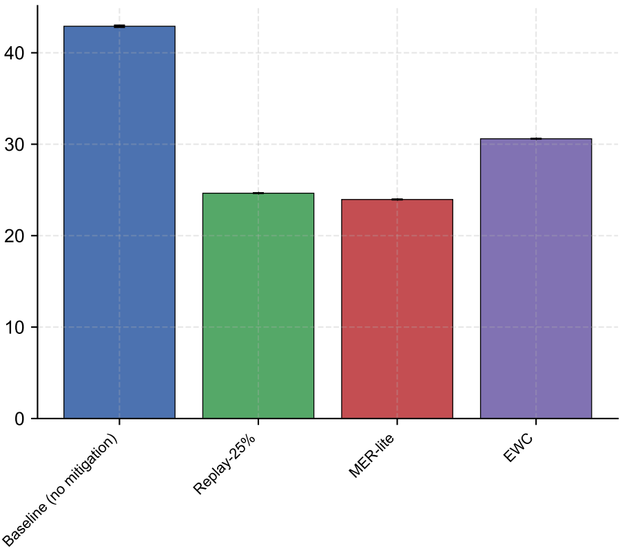
PPL on Domain A (↓ better retention)
