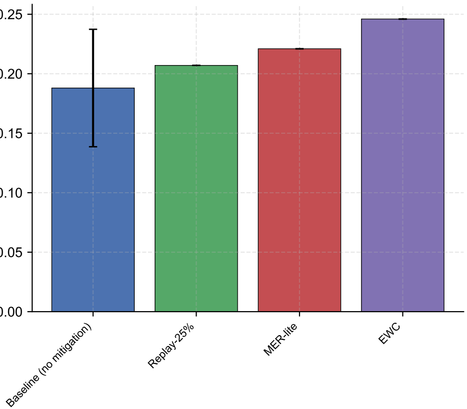
LAMBADA Accuracy (↑ better)
