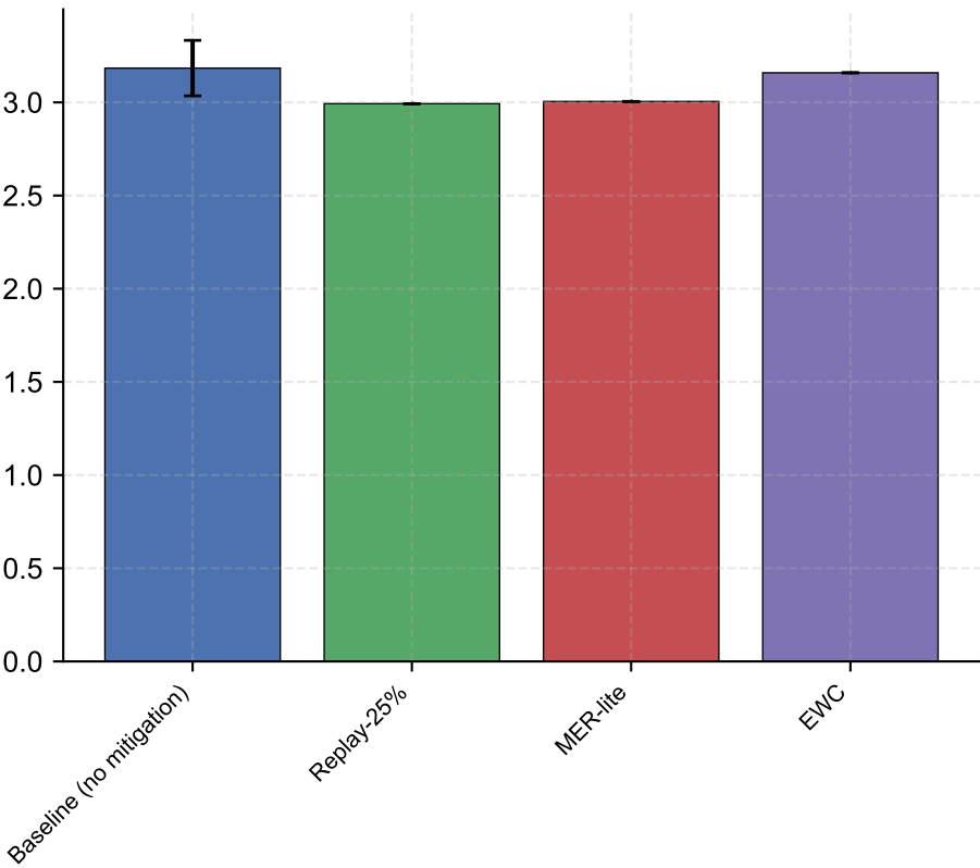
Total Time (hours) (↓ better)
