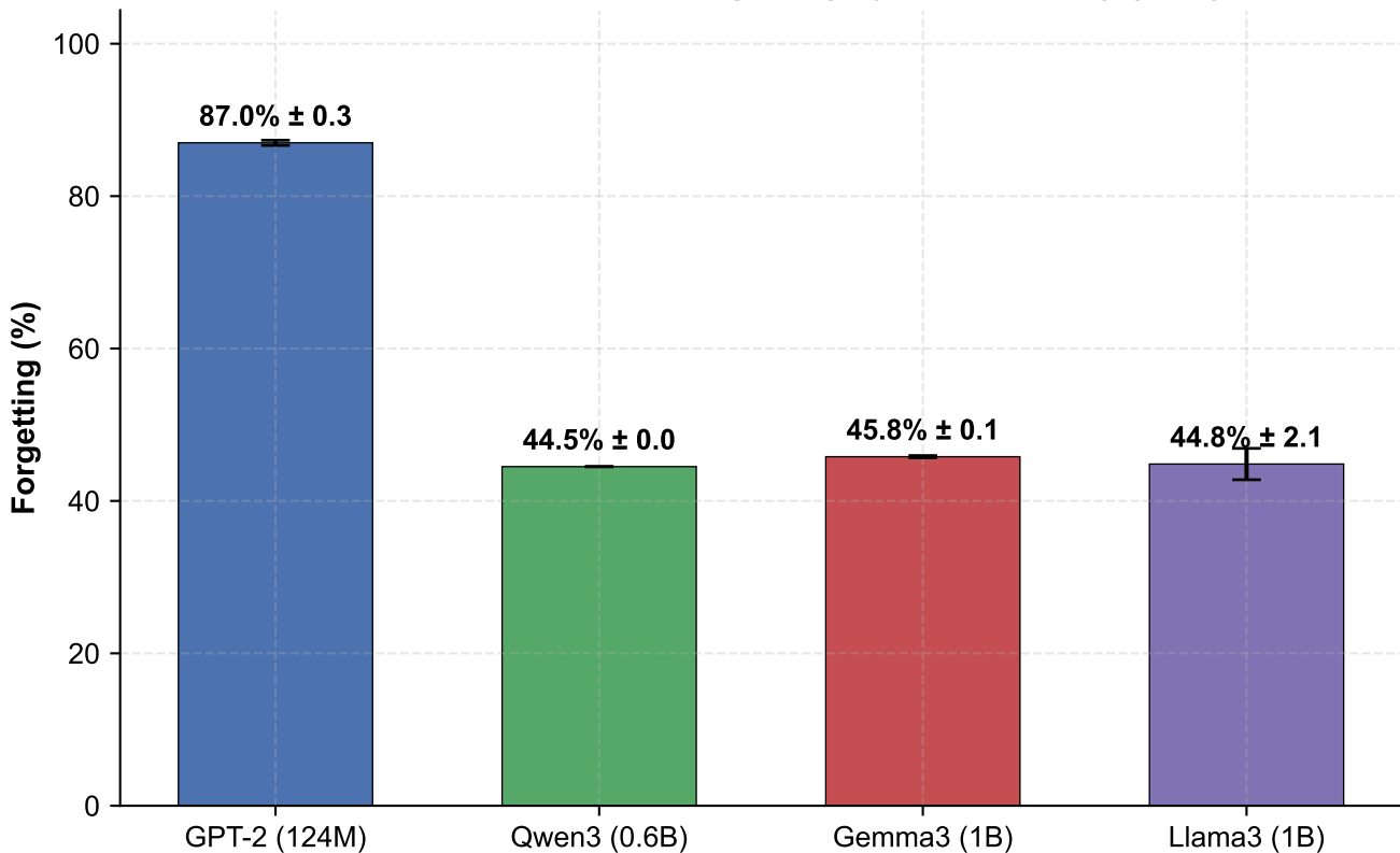
Baseline Catastrophic Forgetting by Model Family (RQ1)
