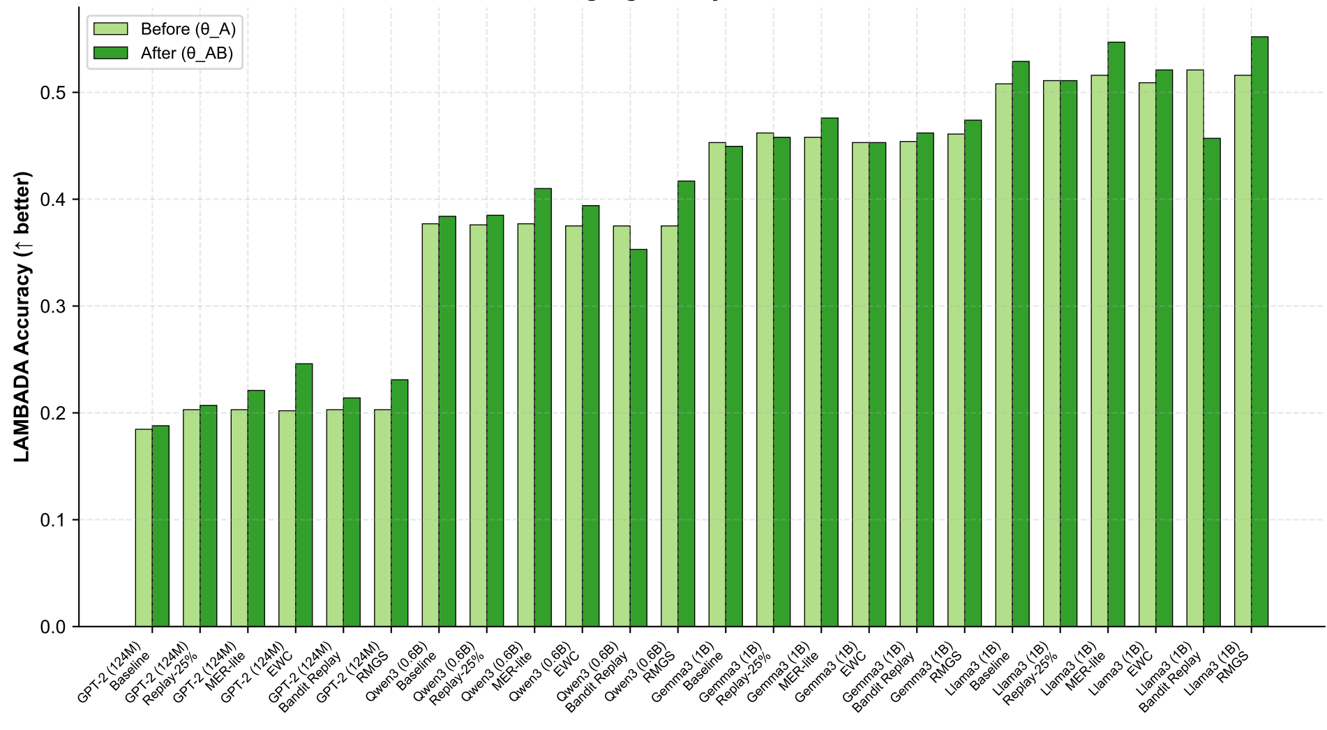
General Language Ability: Before vs After CPT
