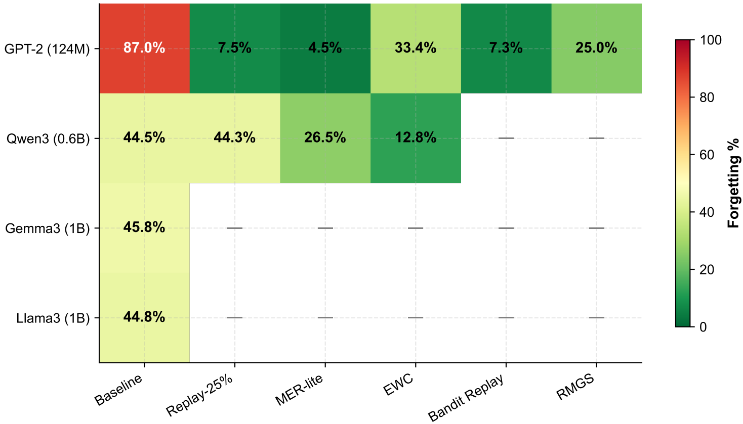
Forgetting % by Model × Method
