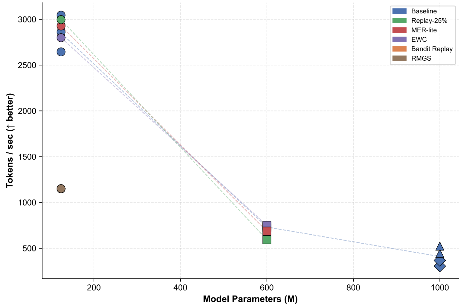
Compute Throughput vs Model Scale
