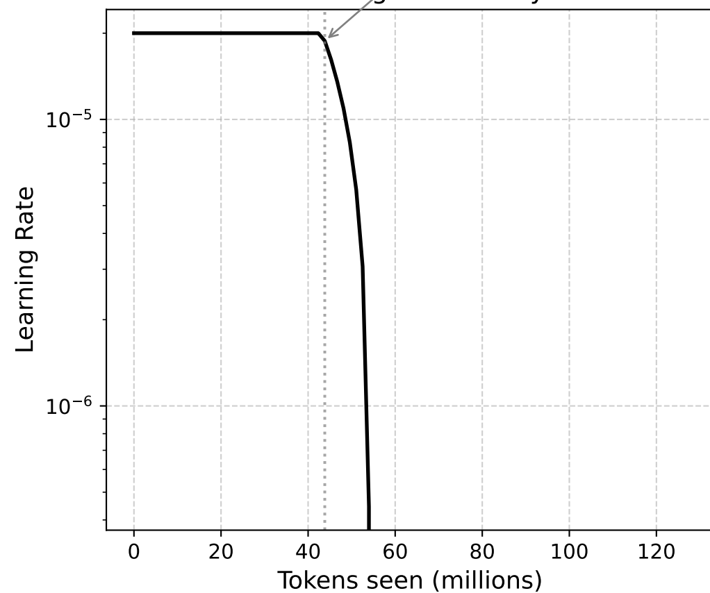
Learning Rate Decay
