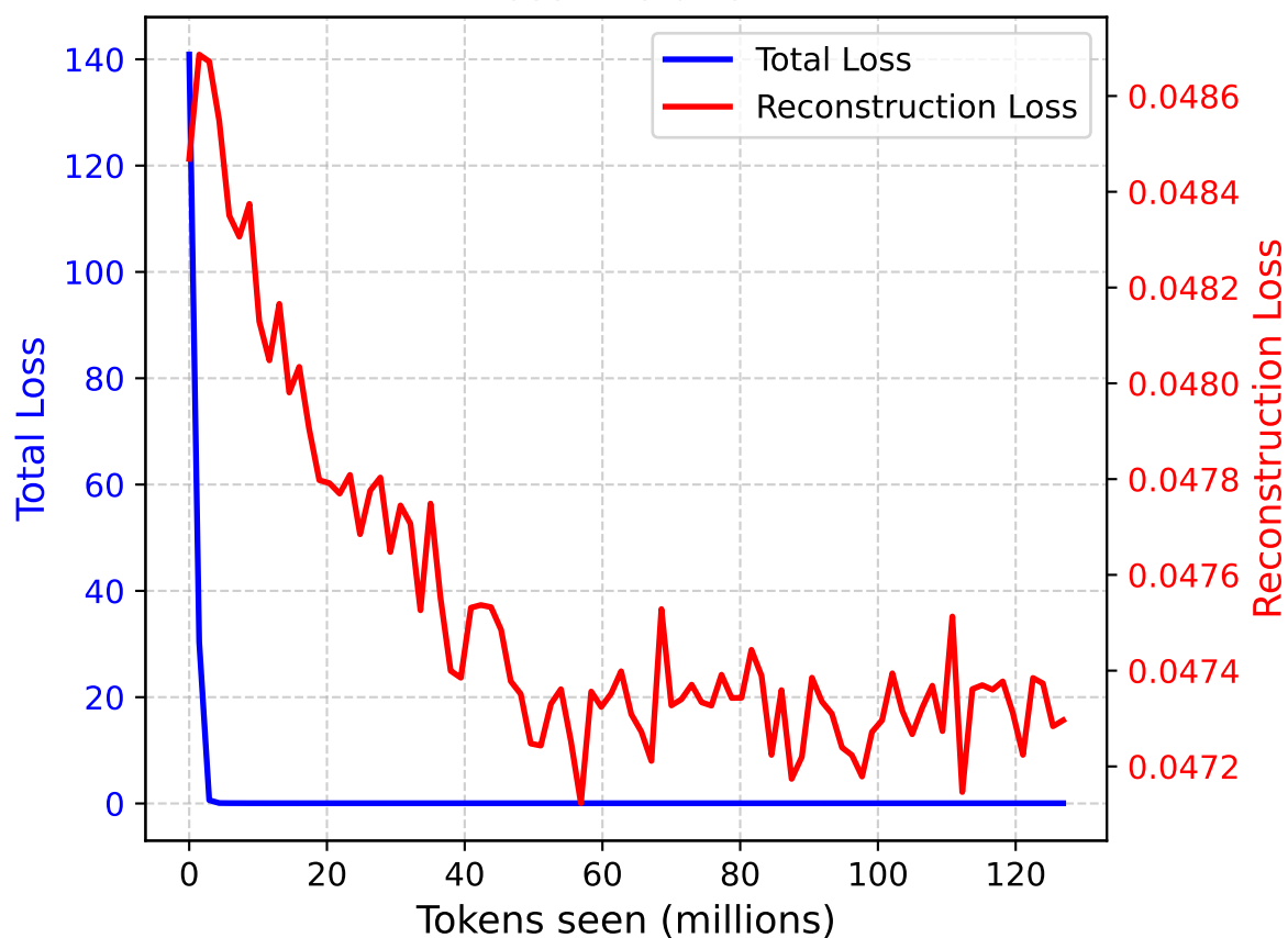
Loss Evolution
