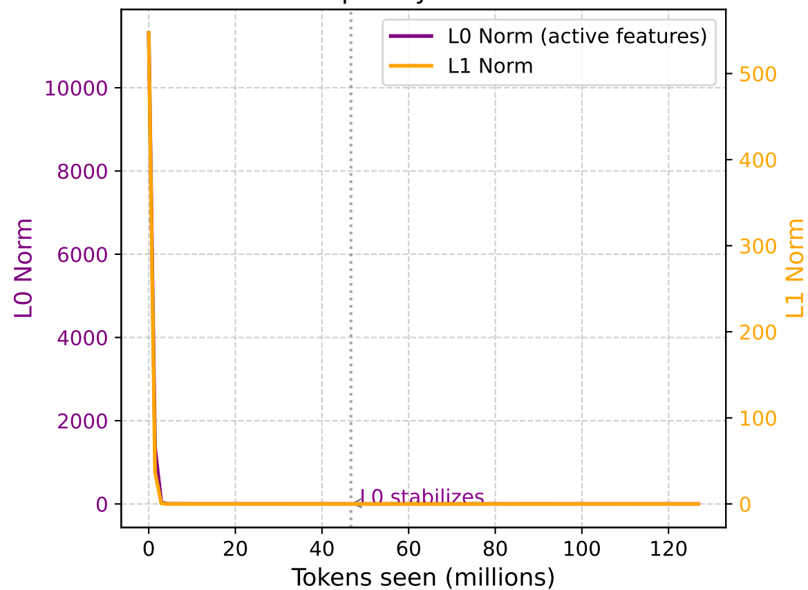
Sparsity Norms
