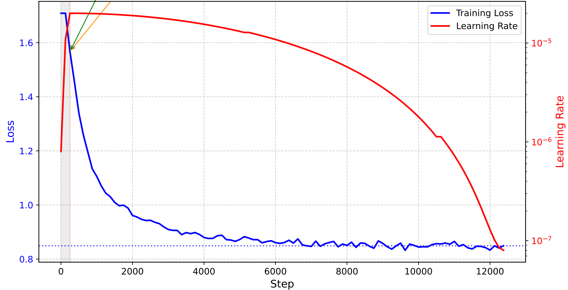
Distillation Training: Loss and Learning Rate
