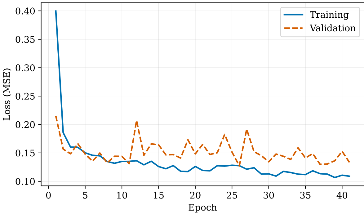
Training History - TRANSFORMER
