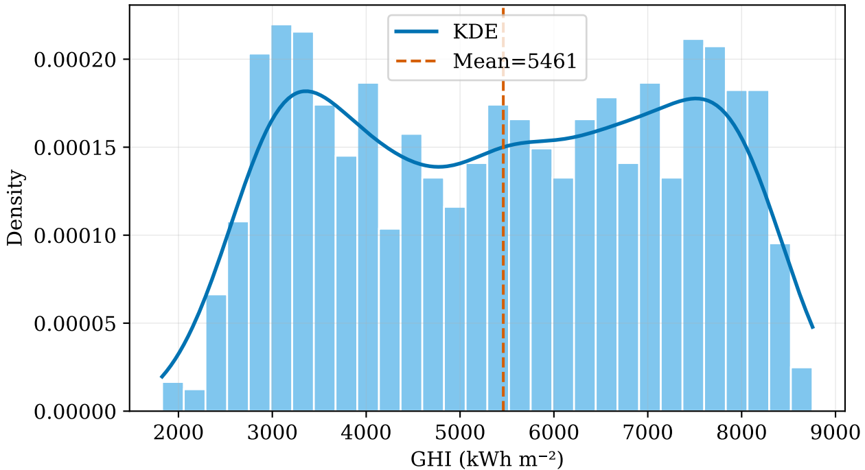
GHI Distribution
