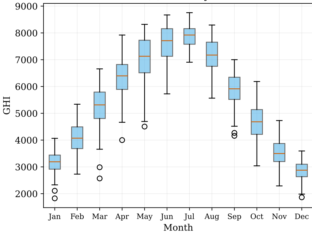
(a) Monthly
