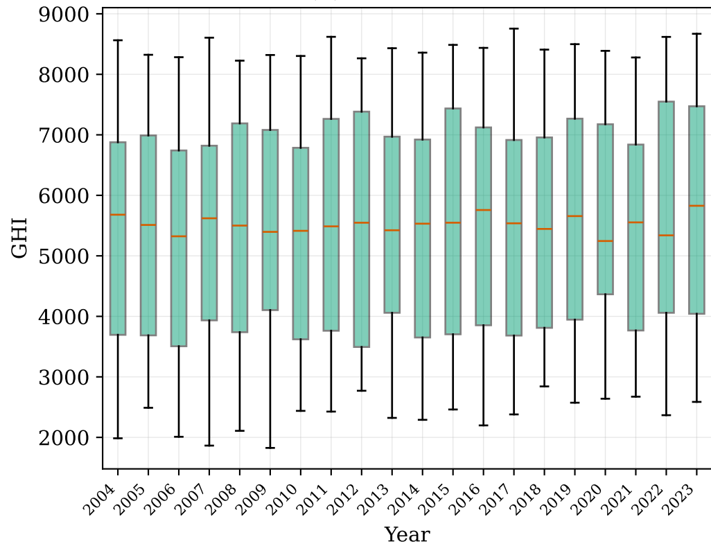
(b) Inter-Annual
