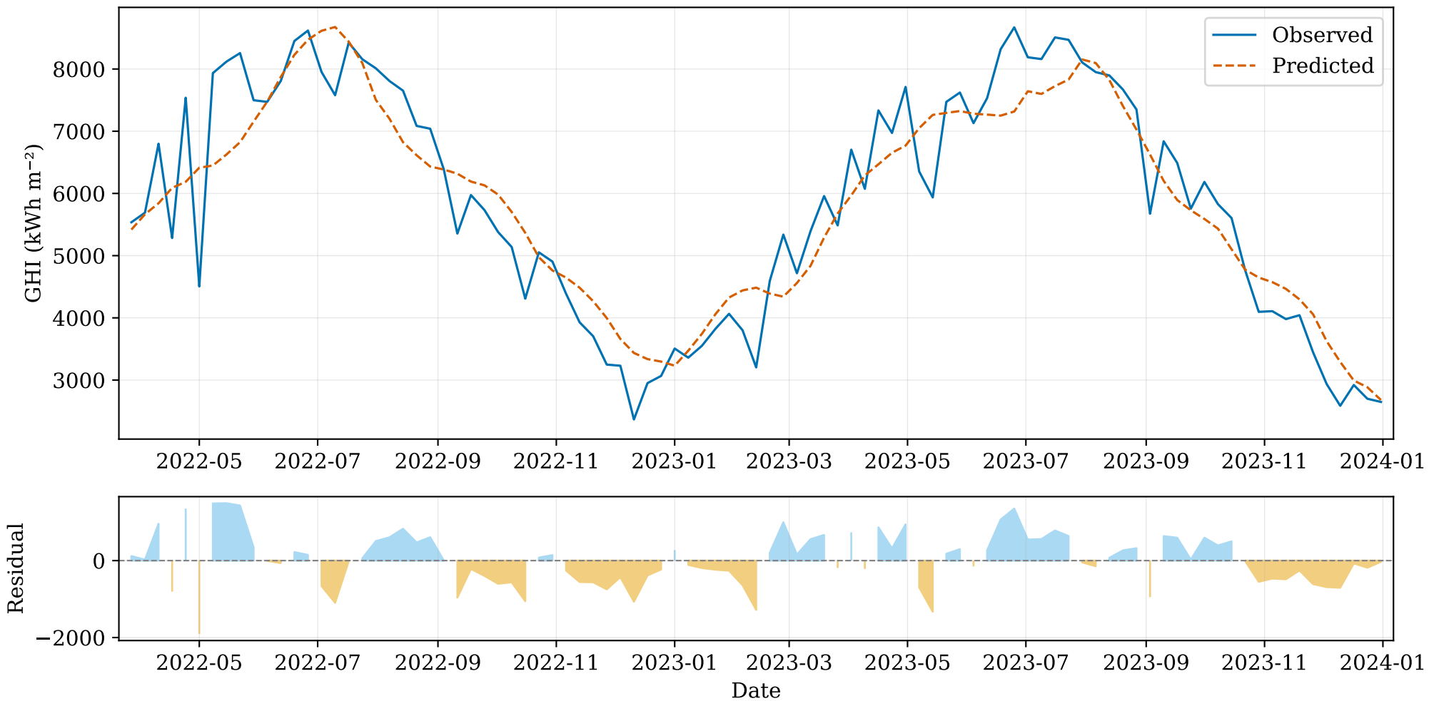
Predictions - LSTM
