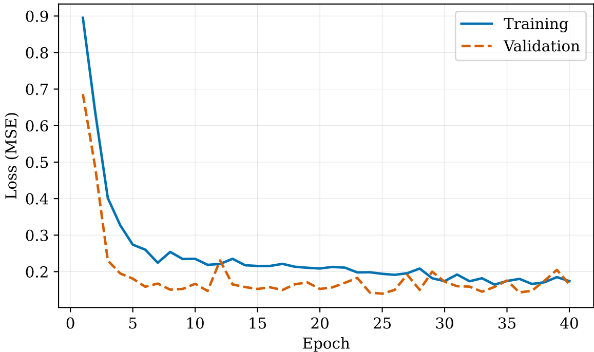
Training History - LSTM
