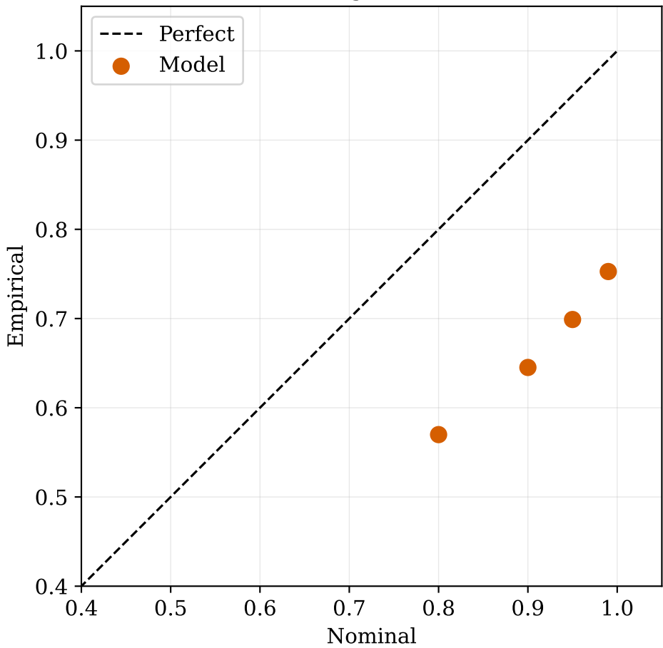
Coverage - LSTM
