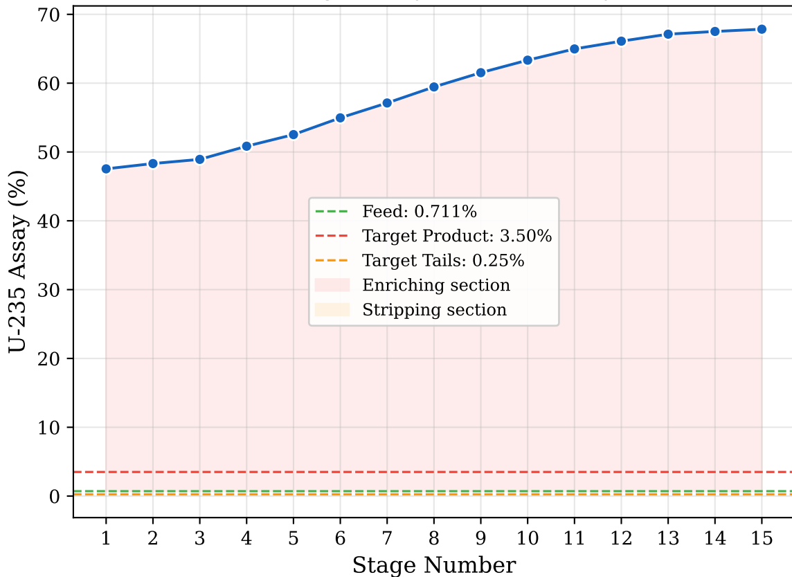
Cascade Stage Assay Profile (Steady State)
