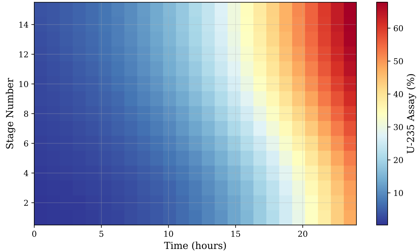
Dynamic Cascade Assay Evolution
