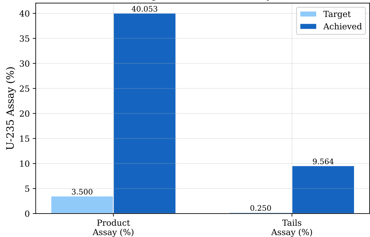
Target vs Achieved Assay
