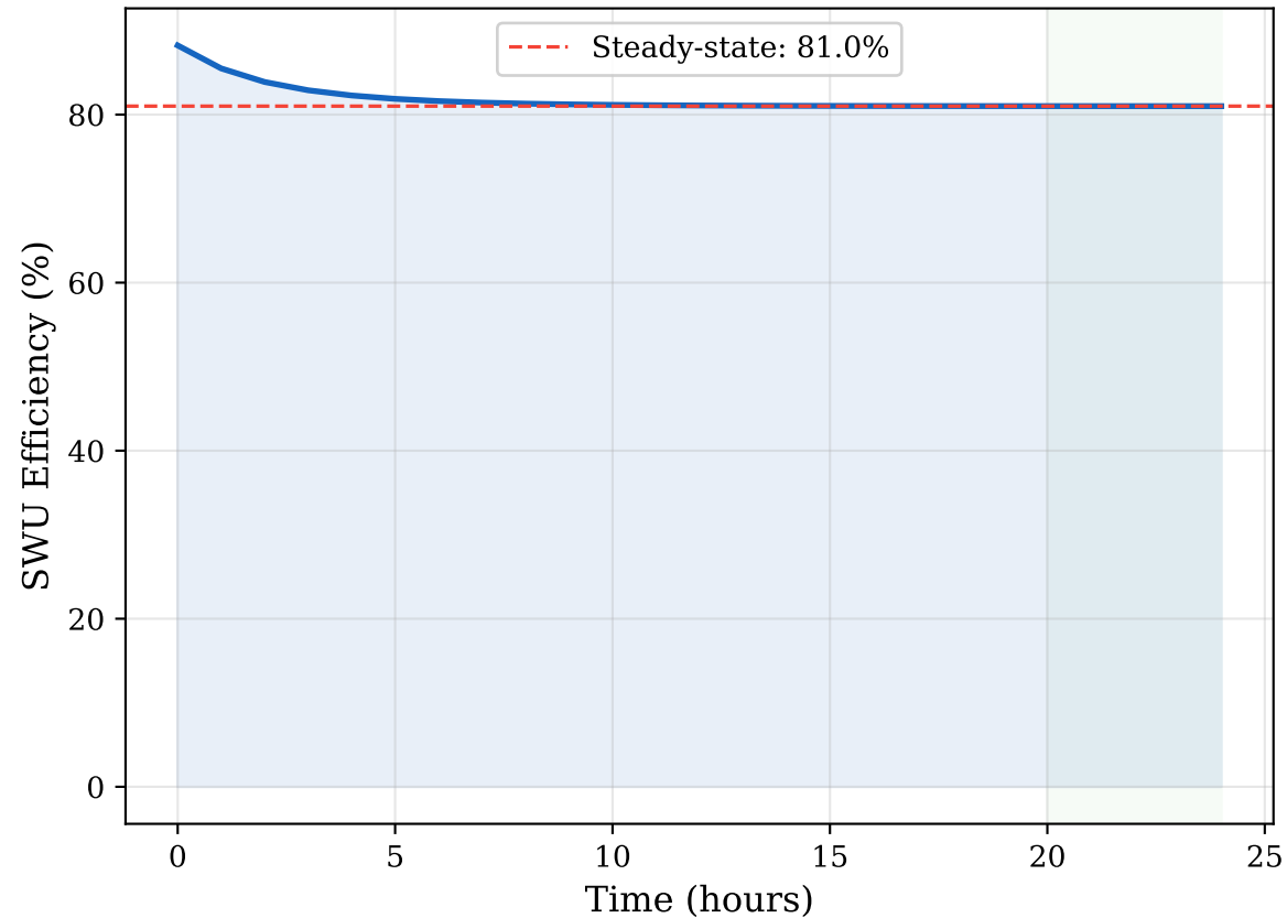
Separative Work Unit Efficiency Over Time
