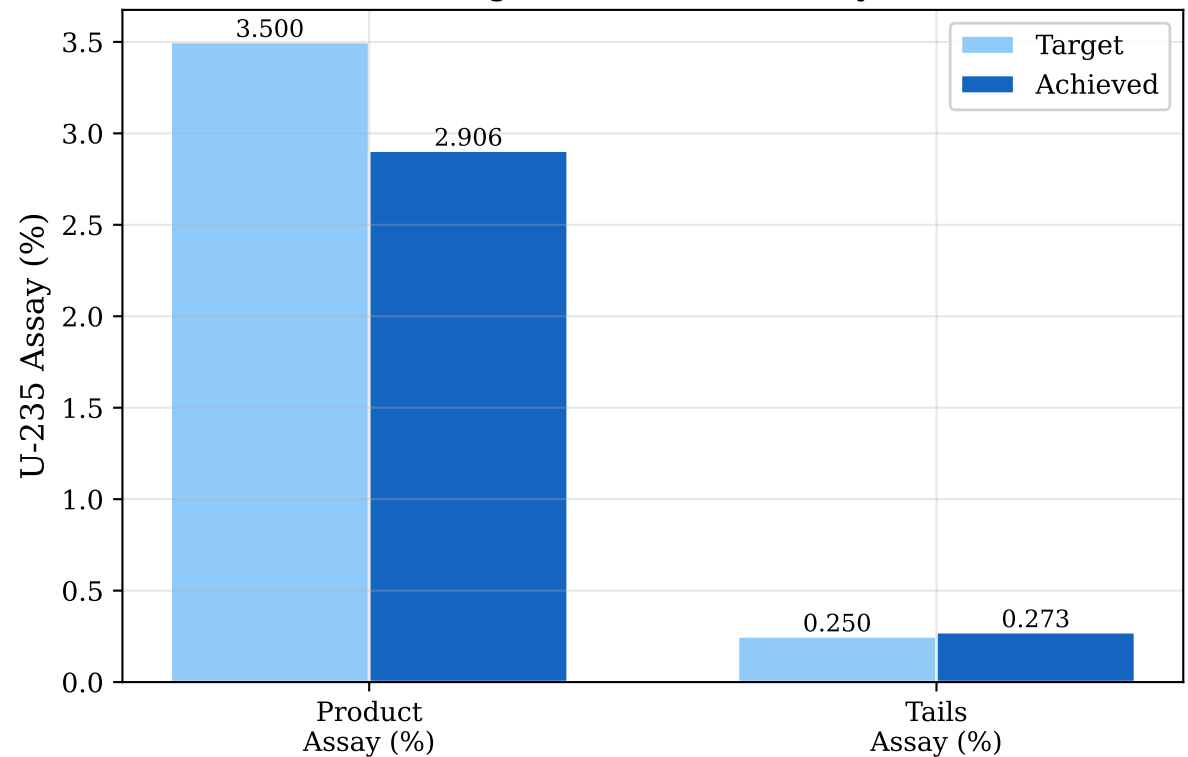
Target vs Achieved Assay
