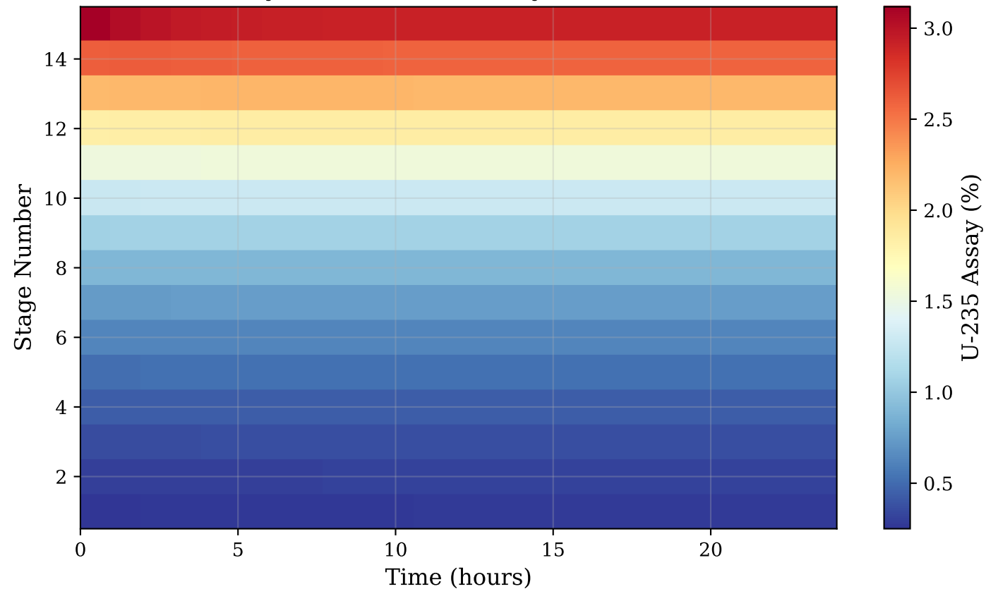
Dynamic Cascade Assay Evolution
