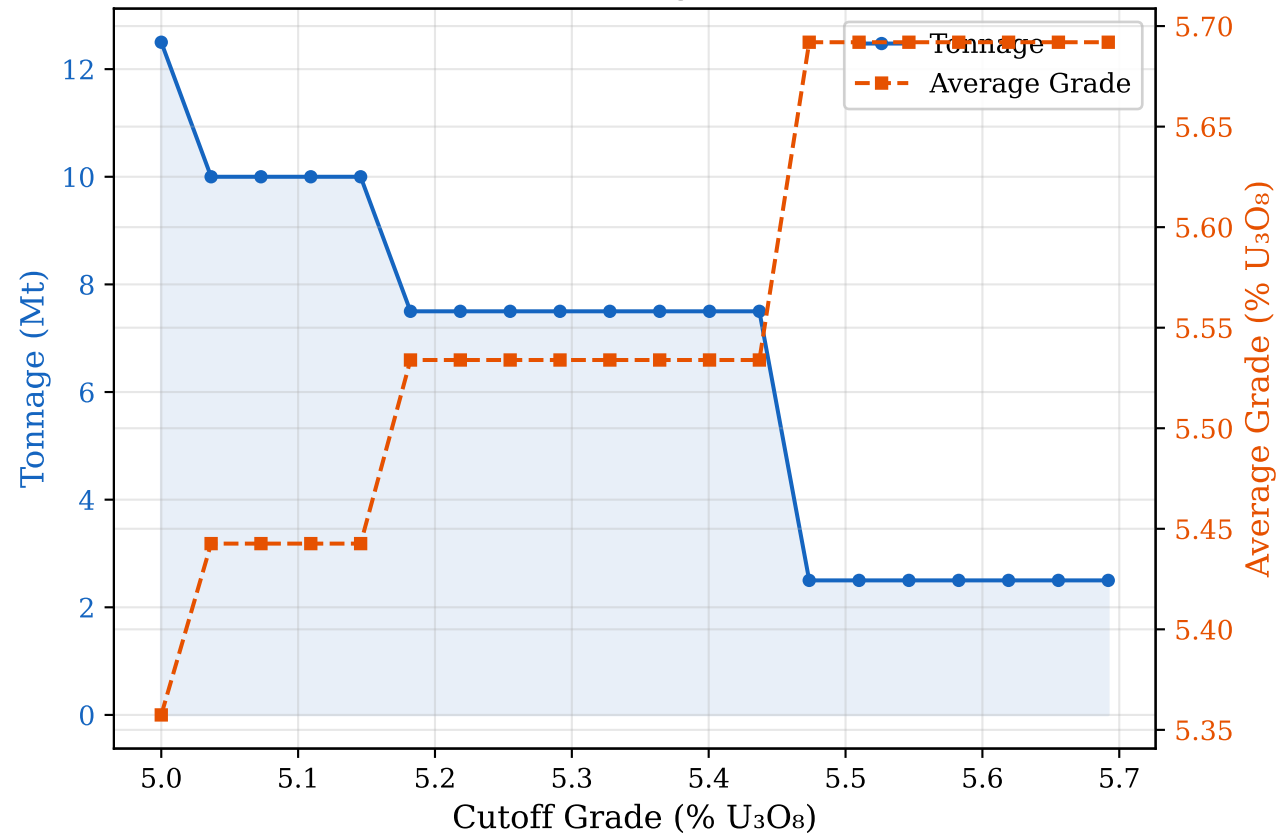
Grade-Tonnage Curve
