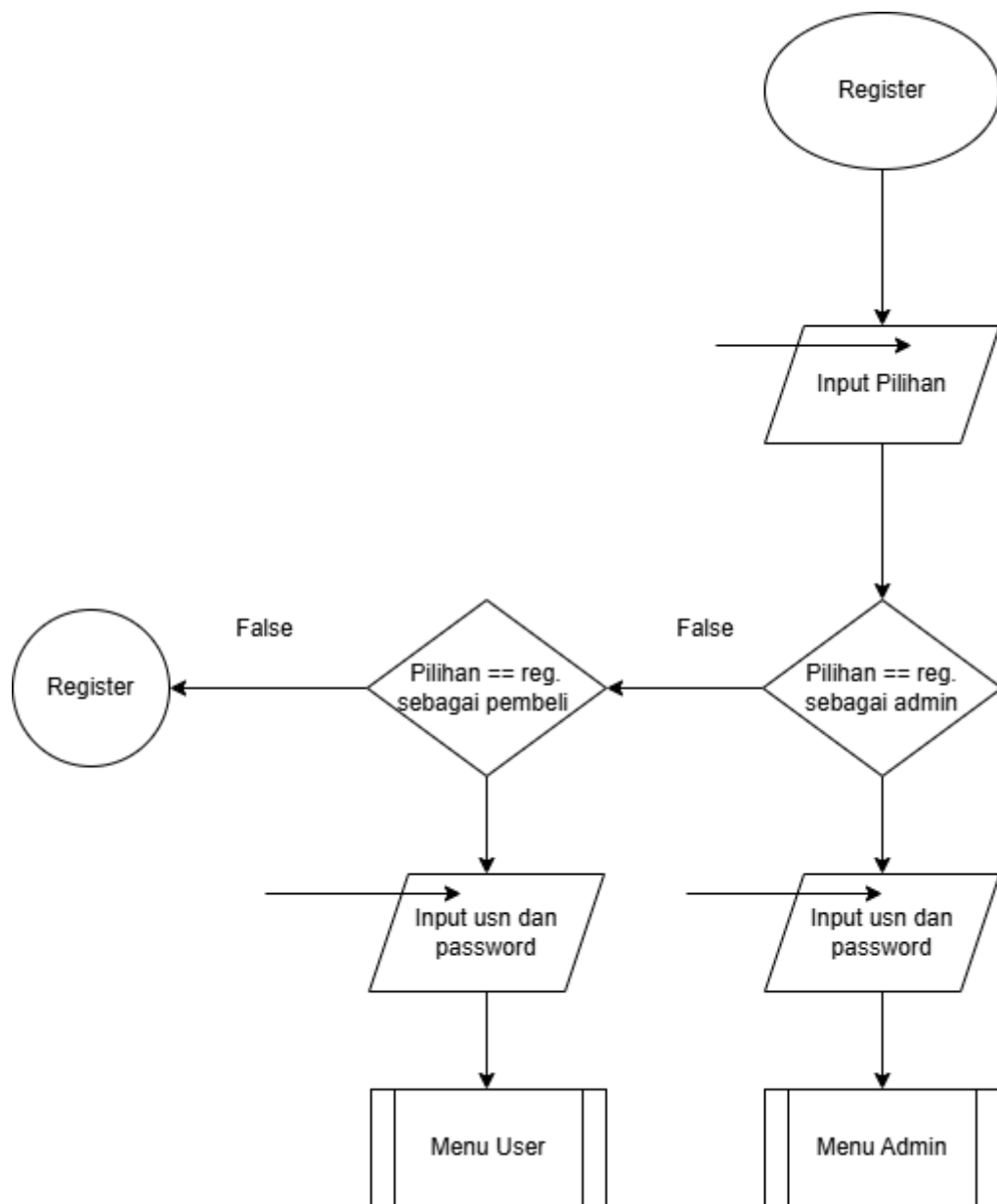
Gambar 2.2 Flowchart Register
