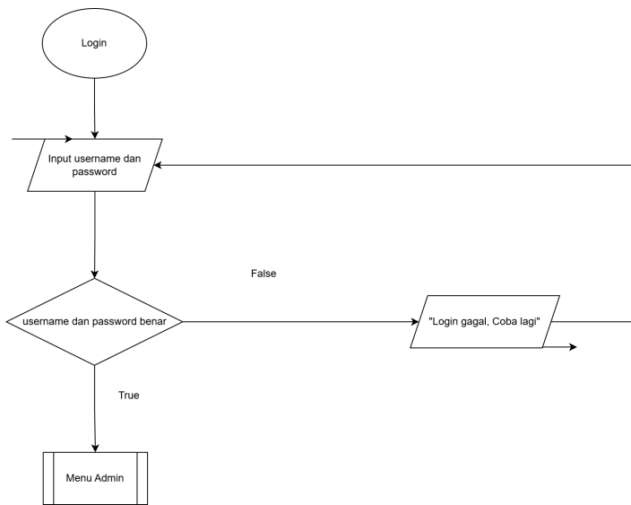
Gambar 2.3 Flowchart Login
