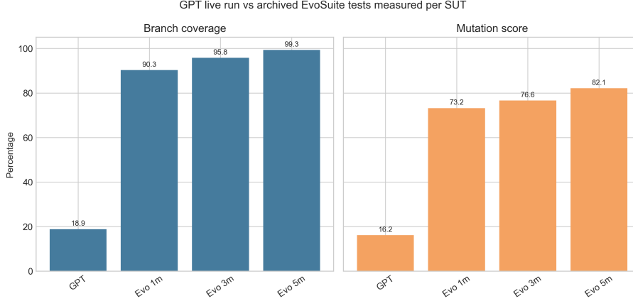
Fig. 3. Pass-conditioned paired GPT-EvoSuite comparison.
