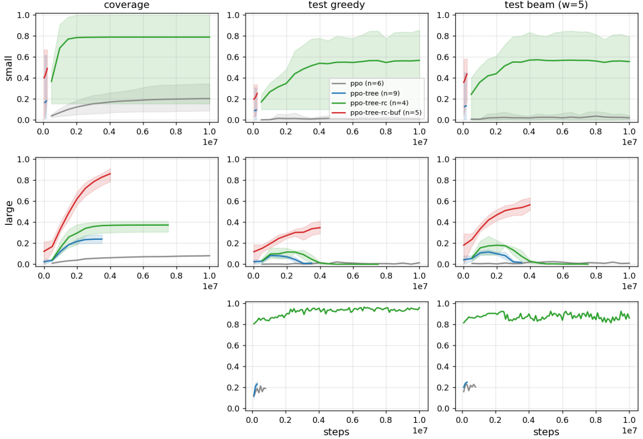
Learning curves for closed equations (mean \pm min/max across seeds)
