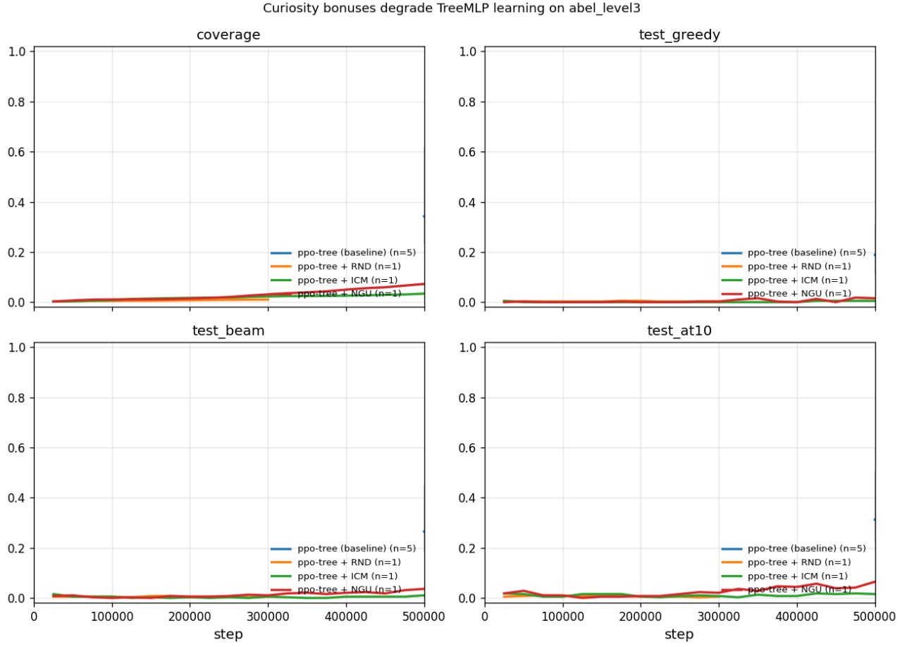
Figure 10. Curiosity bonuses (ICM, NGU, RND) degrade TreeMLP learning on abel_level3. All four panels (coverage, greedy, beam, success@10) at the same training budget ( 5 \times 10^5 steps) show every curiosity variant tracking below the no-curiosity baseline. RND in particular fails to make meaningful progress. Baseline is mean \pm min/max across n=5 seeds; curiosity variants are single seed.
