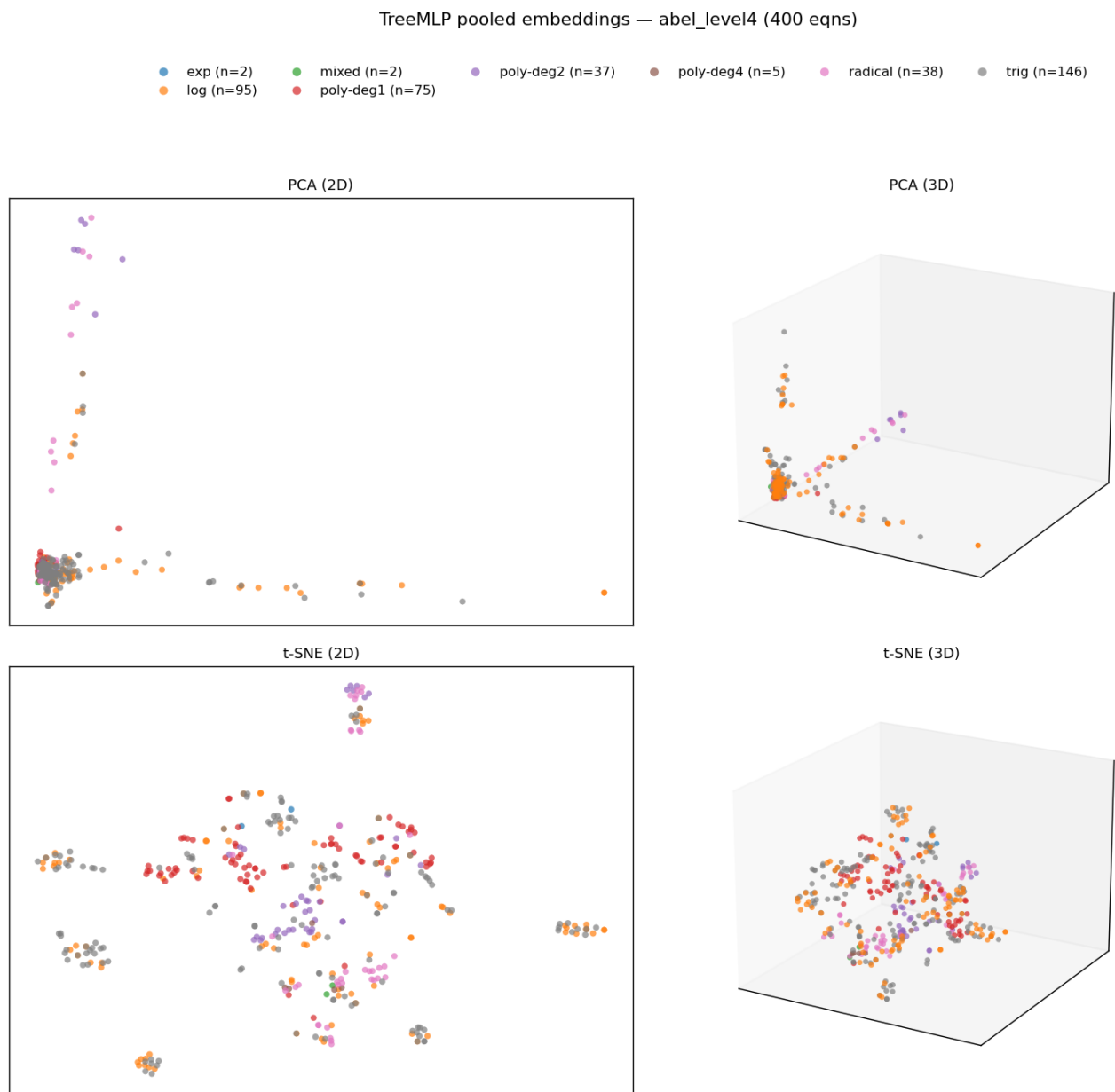
Figure 6. Same as Figure ?? but on the large dataset (depth < 5 ). More types are present and cluster boundaries are softer, consistent with the lower per-type accuracies reported in the main text.
