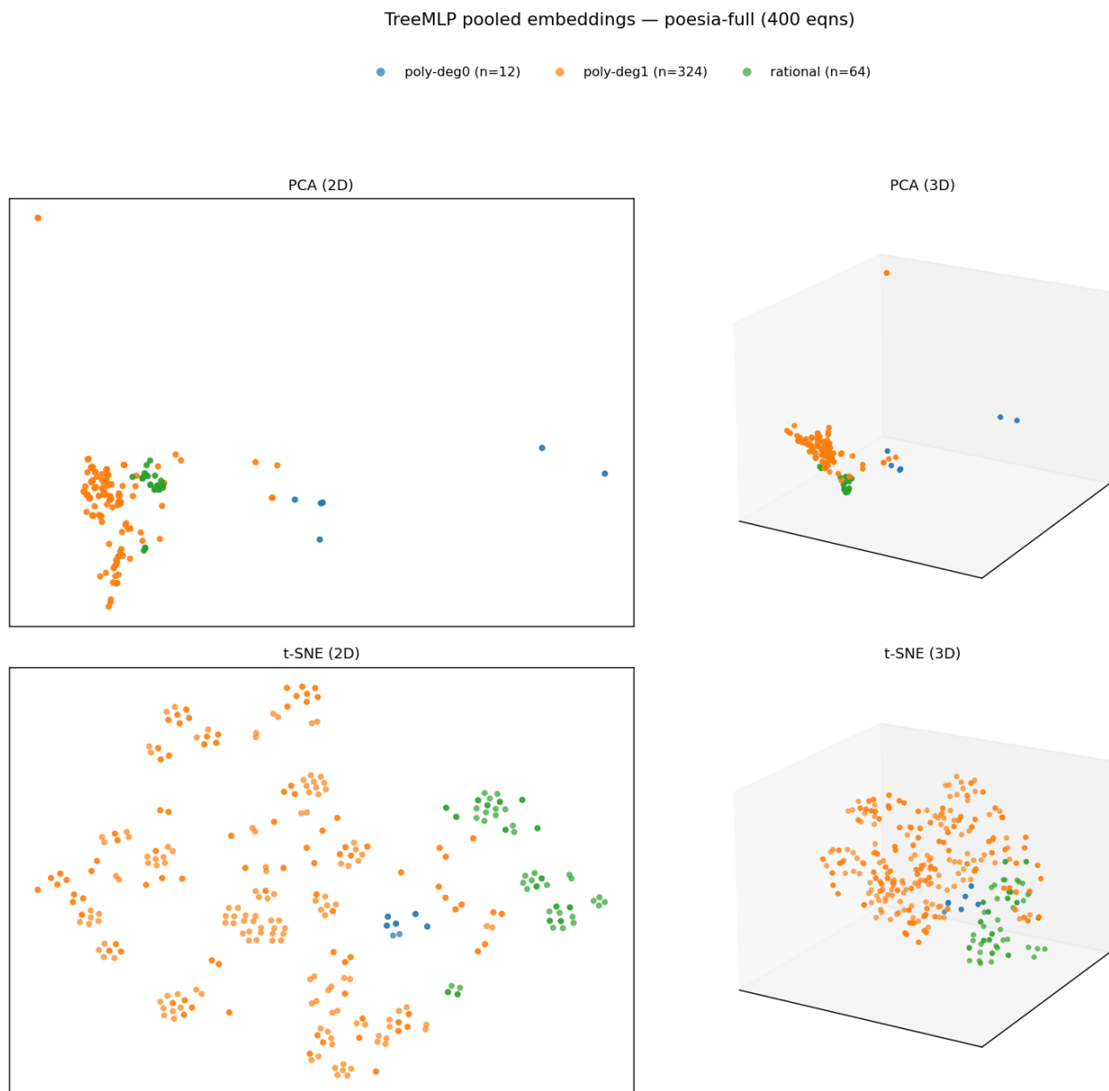
Figure 7. Same as Figure ?? but on CommonCore (poesia). The dataset is dominated by linear and rational equations, giving a simpler embedding geometry.
