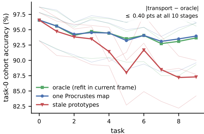
(a) a single rotation tracks the oracle at every depth
