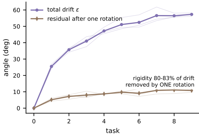
(b) the drift saturates and stays rotational
