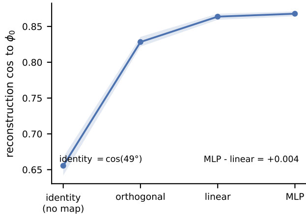
(a) the drift is affine: MLP buys nothing
