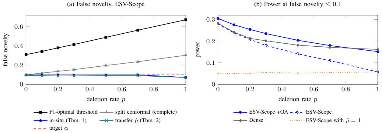
Fig. 2. (a) False novelty of ESV-Scope as witness documents are deleted, mean over 500 random splits. Only the certified rules stay at the target \alpha = 0.1 (dashed). (b) Power of certified rules with transfer calibration, and the worst-case rule \hat{p} = 1 for comparison.
