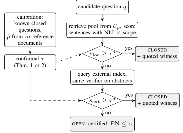
Fig. 1. Certified gap declaration. Shaded boxes are outputs. The threshold \tau is calibrated once and shared by both checks, so the combined score \max\{s_{\text{loc}}, s_{\text{ext}}\} is compared with a single \tau .
