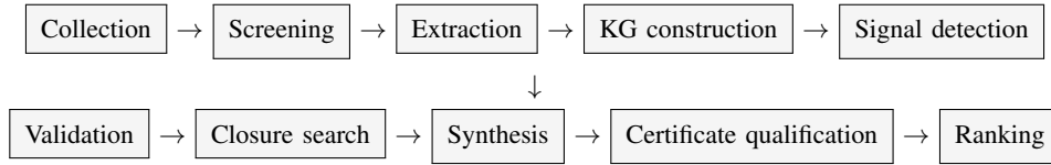
Fig. 1. Ten-stage ESV-Gap pipeline. Detection proposes signals; ranking orders reported candidates but cannot override validation, closure, synthesis, or certificate conditions.
