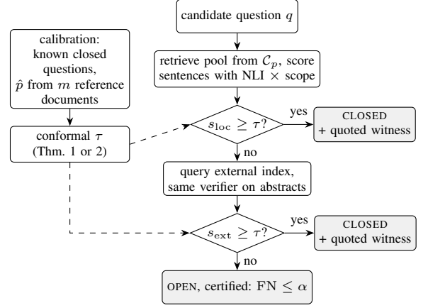
Fig. 1. Certified gap declaration. Shaded boxes are outputs. The threshold \tau is calibrated once and shared by both checks, so the combined score \max\{s_{\text{loc}}, s_{\text{ext}}\} is compared with a single \tau .
