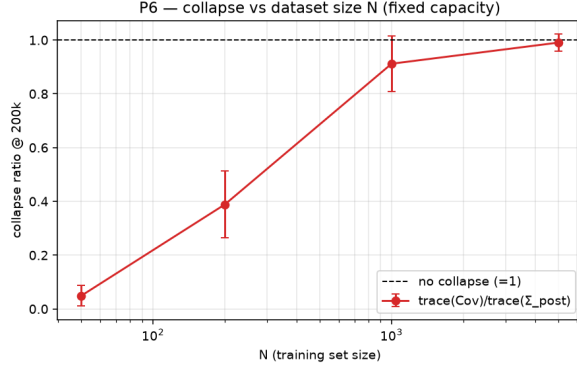
(a) P6: collapse ratio vs. dataset size N .
