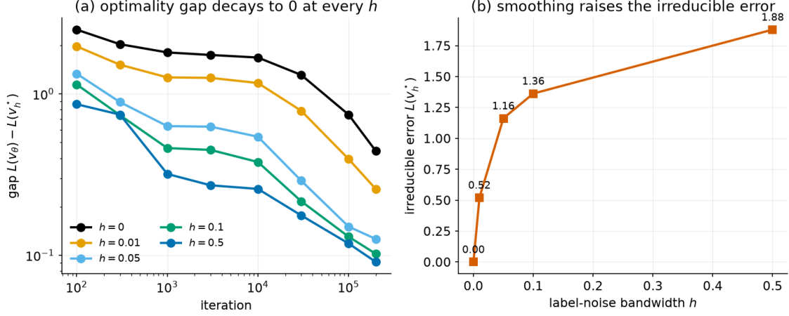
(a) Optimality gap L(v_\theta) - L(v_h^*) decays monotonically to 0 at every h (left); smoothing raises the irreducible error L(v_h^*) (right).
