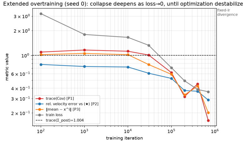
Figure 3: Extended seed-0 trajectory: \text{tr Cov} , velocity error, \|\text{mean} - x^i\| and the training loss decrease together, identifying P1–P3 as one phenomenon driven by loss \rightarrow 0 (the exact minimiser has loss 0).
