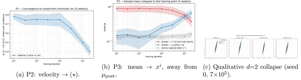
Figure 2: The remaining EXP-1 observables. The learned velocity approaches the collapsed closed form (\star) (a) and the generated mean migrates from the Bayes posterior mean to the memorised training point (b); in two dimensions the sample cloud that initially fills the posterior ellipse contracts to a point (c). All descend in lockstep with P1.
