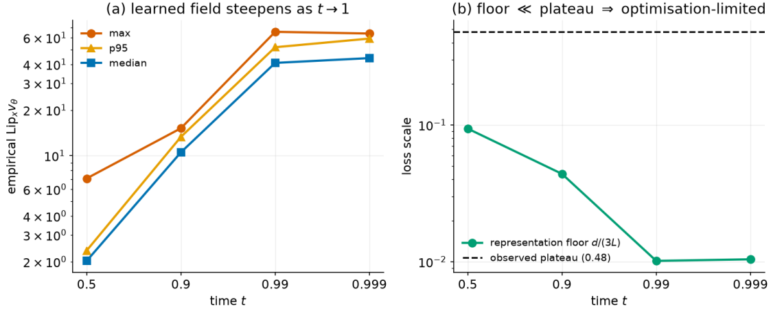
(b) The empirical Lipschitz constant of v_\theta blows up as t \rightarrow 1 (left); the representation floor d/(3L) is \sim 50\times below the observed loss plateau (right), so the plateau is optimisation-limited.
