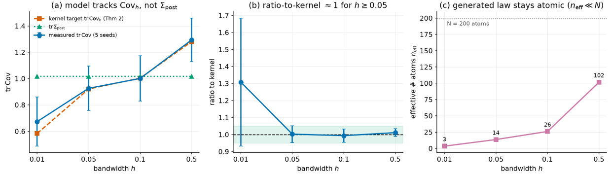
Figure 5: P7 headline (5 seeds, error bars over seeds). (a) The generated \text{tr Cov} follows the kernel target \text{tr Cov}_h (dashed) and crosses \text{tr } \Sigma_{\text{post}} (dotted, flat) only incidentally near h=0.1 . (b) The ratio-to-kernel lies within the shaded [0.95, 1.05] band for h \geq 0.05 . (c) n_{\text{eff}} \ll N : the endpoint law is a sparse mixture of training atoms (Proposition 6), not a continuous posterior.
