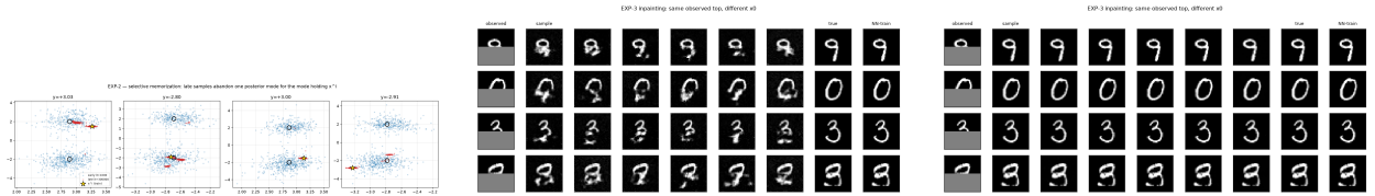
(a) EXP-2: samples abandon one posterior mode. (b) EXP-3, iter 200: diverse completions. (c) EXP-3, iter 15000: identical, memorised.
