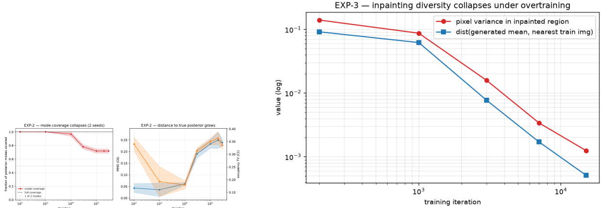
(a) EXP-2: mode coverage \rightarrow single mode. (b) EXP-3: inpainting variance / NN-distance collapse.
