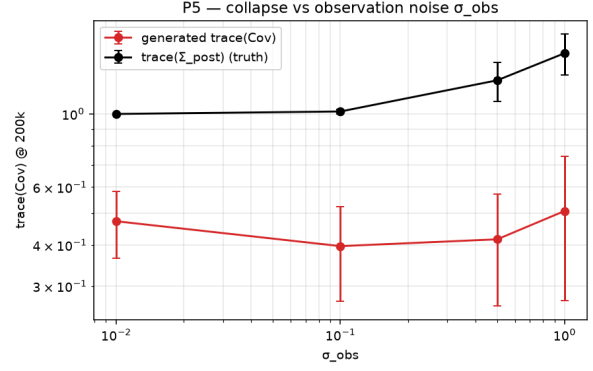
(b) P5: collapse ratio vs. observation noise \sigma_{\text{obs}} .
