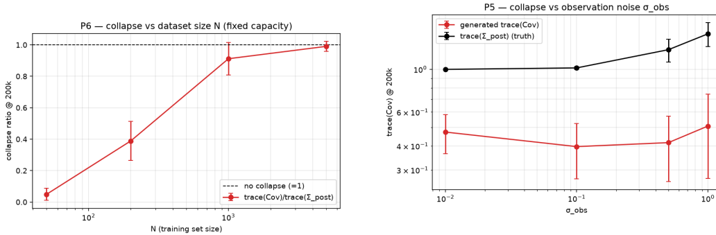
(b) P5: generated \text{tr Cov} and \text{tr } \Sigma_{\text{post}} vs. \sigma_{\text{obs}} (their ratio is the collapse ratio of Table 7).
