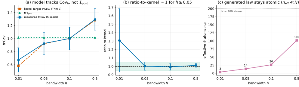
Figure 1: P7 headline (5 seeds, error bars over seeds). (a) Generated \text{tr Cov} follows the kernel target \text{tr Cov}_h (dashed) and crosses \text{tr } \Sigma_{\text{post}} (dotted) only incidentally near h=0.1 . (b) Ratio-to-kernel stays in the shaded [0.95, 1.05] band for h \geq 0.05 . (c) n_{\text{eff}} \ll N : a sparse mixture of atoms (Proposition 6), not a continuous posterior.
