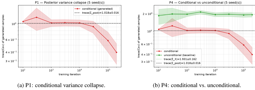
Figure 8: Overtraining collapses the conditional generated variance toward zero, while the unconditional model retains data-scale variance (Corollary 1).
