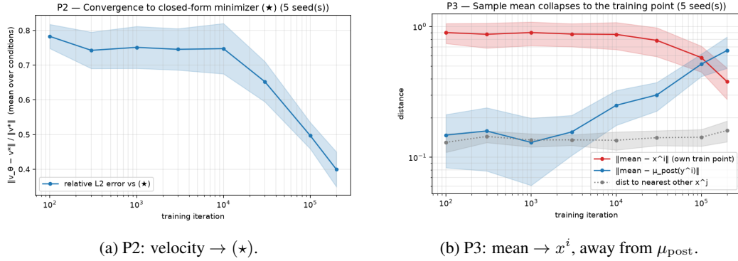
Figure 9: The learned velocity approaches the collapsed closed form ( \star ) (a) and the generated mean migrates from the Bayes posterior mean to the memorised training point (b). Both descend in lockstep with P1. Panel (b) also plots the distance from x^i to the nearest other training point (dotted, \approx 0.17 ) as a scale reference: at 2 \times 10^5 iterations \|\text{mean} - x^i\| = 0.38 still exceeds it, so the mean has not yet resolved x^i from its neighbours at this budget—it does so in the extended run (0.137 at 10^6 ), and the per-sample memorisation ratio of Figure 12 makes the same point without relying on this scale.
