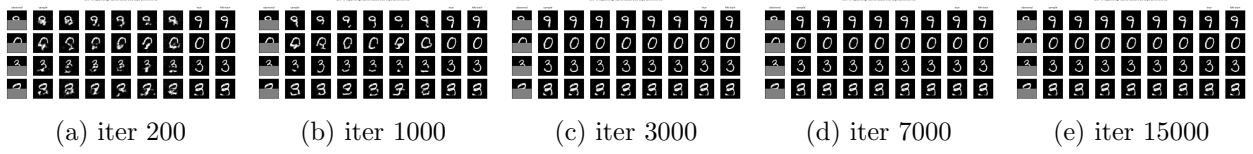
Figure 10: EXP-3 collapse trajectory (MNIST inpainting). Each grid shows completions of a fixed masked digit from different source samples x_0 . Early in training (iter 200) the completions are diverse—a calibrated conditional sampler; as the loss descends they sharpen progressively (iter 1000–7000) and, by iter 15000, are identical to one another and equal to the nearest training image (inpaint-region pixel variance 0.140 \rightarrow 0.0013 , a \sim 100\times drop). This is the same loss \rightarrow 0 -paced collapse as EXP-1, on real image data.
