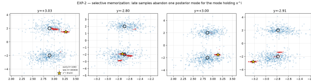
Figure 9: EXP-2 qualitative collapse. Generated samples concentrate on the posterior mode containing the memorised x^i and abandon the other, even though the analytic posterior for this observation is bimodal.
