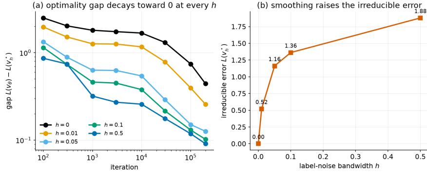
Figure 3: Optimality gap L(v_\theta) - L(v_h^*) decays monotonically toward 0 at every h (left)—it is still positive at the last checkpoint (0.09–0.44), which is the optimisation gap of Section 5; smoothing raises the irreducible error L(v_h^*) (right).
