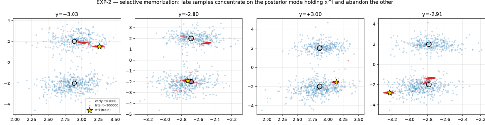
Figure 15: EXP-2 qualitative collapse (seed 0, 3 \times 10^5 iterations). Early samples (blue) cover both modes of the bimodal analytic posterior; late samples (red) concentrate on the mode containing the memorised x^i and abandon the other. Assigning late samples to their nearest posterior mode, the share landing in the x^i -containing mode is 0.999, 0.766, 0.990 and 1.000 for the four conditions shown (versus \approx 0.5 each at iteration 10^3 ). The one condition that retains 23% of its mass on the abandoned mode shows that this is an optimisation-paced process (Section 5), consistent with the aggregate mode coverage of Section 4.3 settling at 0.72 rather than at the single-mode value 0.5.
