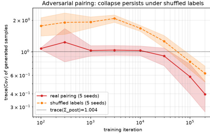
Figure 11: \text{tr Cov} under the real EXP-1 pairing (5 seeds, as in Fig. 6) vs. the same architecture and schedule trained on Y randomly permuted relative to X (5 seeds). Both collapse monotonically well below \text{tr } \Sigma_{\text{post}} ; the shuffled run lags the real pairing at 2 \times 10^5 iterations ( 0.625 \pm 0.108 vs. 0.396 \pm 0.127 )—an optimisation-gap difference, not a failure of Proposition 2, whose population target is 0 either way.
