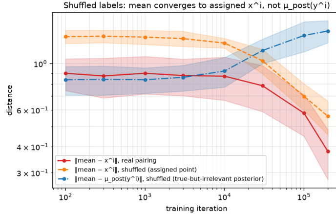
Figure 12: Under shuffled labels, the generated mean converges to the assigned training point x^i ( \|\text{mean} - x^i\| : 1.35 \pm 0.10 \rightarrow 0.559 \pm 0.104 ) while moving away from the true analytic posterior mean of that y^i ( \|\text{mean} - \mu_{\text{post}}(y^i)\| : 0.84 \pm 0.13 \rightarrow 1.437 \pm 0.176 )—the two curves cross between 10^4 and 3 \times 10^4 iterations. Under the real pairing the corresponding gap is far smaller ( \|\text{mean} - \mu_{\text{post}}\| = 0.656 \pm 0.177 at 2 \times 10^5 , Table 1), since there x^i and \mu_{\text{post}}(y^i) are close by construction.
