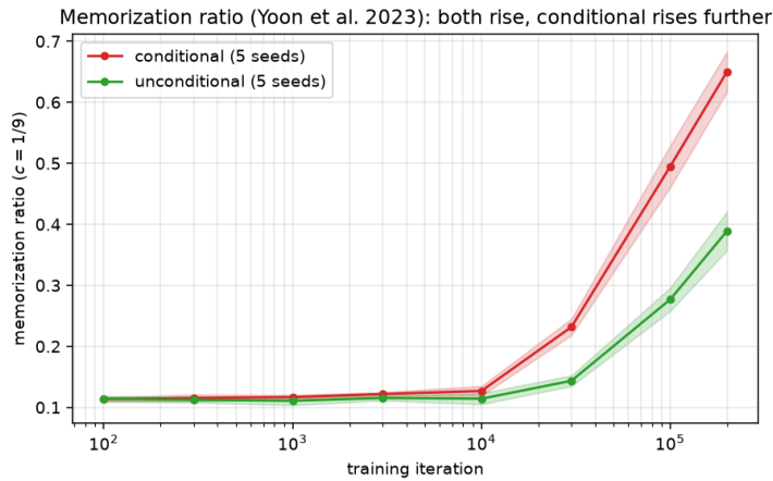
Figure 10: Memorisation ratio (5 seeds each) for the same conditional and unconditional EXP-1 runs as Figure 6. Both rise from the common \approx 0.11 baseline of a well-calibrated sampler; the conditional ratio rises higher ( 0.650 \pm 0.033 at 2 \times 10^5 ) than the unconditional one ( 0.389 \pm 0.032 ), consistent with single-atom vs. full-empirical-measure memorisation (Corollary 1).
