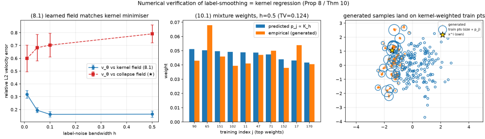
Figure 13: Kernel-theory verification: the learned field matches the kernel minimiser (3) (left); the predicted atom weights p_i^{(h)} \propto K_h match the empirical nearest-atom assignment (centre); and, for one condition y , generated samples (orange) land on the training points weighted most heavily by the kernel (blue circles, radius \propto p_i^{(h)} ), confirming Theorem 1’s mixture-over-atoms endpoint law directly in sample space (right). The right panel is at h=0.5 , where the query’s own atom x^i (gold star) is only one of n_{\text{eff}} \approx 102 contributors and therefore carries no special weight—the opposite of the h \rightarrow 0 regime of Corollary 2.
