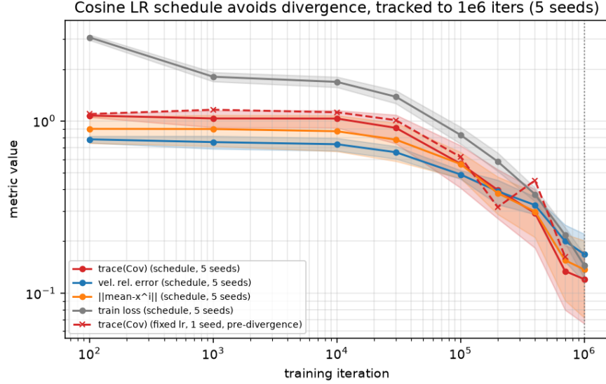
Figure 9: Extended training with a cosine learning-rate schedule (5 seeds, error bars over seeds) tracks all the way to 10^6 iterations without ever diverging, unlike the fixed-lr single seed (dashed), which is cut off at its last pre-divergence checkpoint. On the same seed, the schedule also reaches a lower tr Cov than the fixed-lr run at the matching 7 \times 10^5 checkpoint (0.128 vs. 0.162); the 5-seed mean at 1 \times 10^6 carries enough between-seed spread that it should be read mainly as evidence of stability, not as a precise depth estimate (see main text). tr Cov, velocity error, \|\text{mean} - x^i\| , and the training loss all decrease together throughout, identifying P1–P3 as one phenomenon driven by \text{loss} \rightarrow 0 (the exact minimiser has loss 0).
