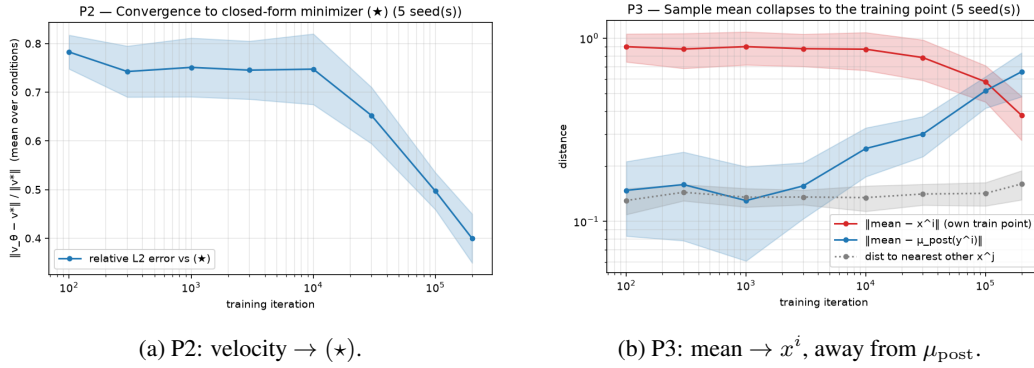
Figure 7: The learned velocity approaches the collapsed closed form (\star) (a) and the generated mean migrates from the Bayes posterior mean to the memorised training point (b). Both descend in lockstep with P1. Panel (b) also plots the distance from x^i to the nearest other training point (dotted, \approx 0.17 ) as a scale reference: at 2 \times 10^5 iterations \|\text{mean} - x^i\| = 0.38 still exceeds it, so the mean has not yet resolved x^i from its neighbours at this budget—it does so in the extended run (0.137 at 10^6 ), and the per-sample memorisation ratio of Figure 10 makes the same point without relying on this scale.
