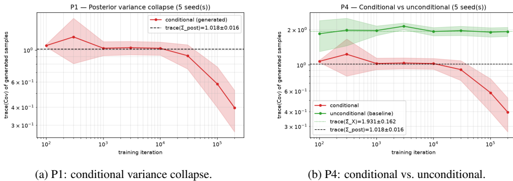
Figure 6: Overtraining collapses the conditional generated variance toward zero, while the unconditional model retains data-scale variance (Corollary 1).
