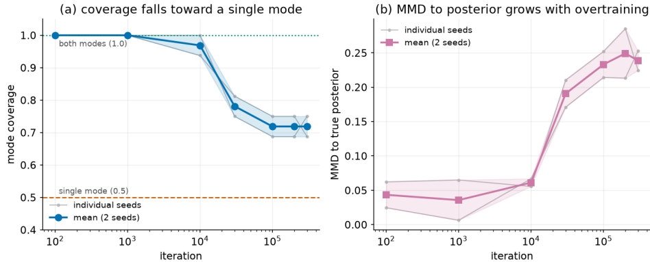
Figure 14: EXP-2 (GMM), mean of 2 seeds with per-seed traces and a \pm std band. (a) Mode coverage holds at 1.0 (both posterior modes) until \sim 10^4 iterations, then falls toward the single-mode line 0.5. (b) The MMD to the true bimodal posterior is near zero in the calibrated phase and grows as overtraining concentrates the samples on one mode. Onset matches EXP-1.
