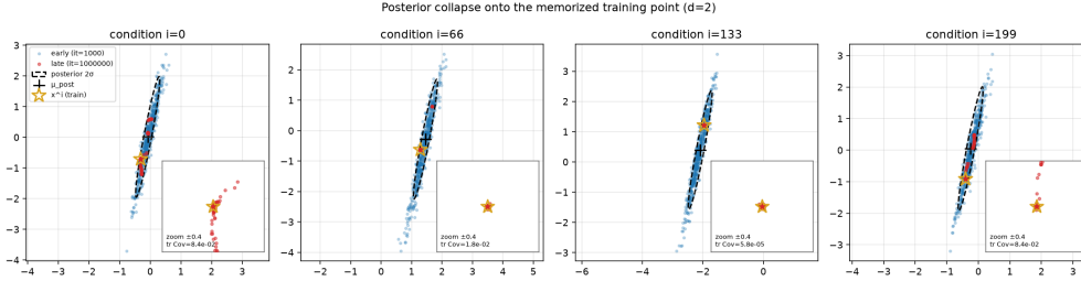
Figure 8: Qualitative d=2 collapse (seed 0, cosine-schedule run at 1 \times 10^6 iterations): the sample cloud that initially fills the posterior ellipse (blue, early, 10^3 iterations) contracts onto the memorised training point (red, late) for four conditions y^i . Because the late cloud is one to four orders of magnitude tighter than the posterior scale, each panel carries an inset zoomed to a fixed \pm 0.4 window around x^i , annotated with that condition’s tr Cov. The collapse is not uniform across conditions at this budget— i=133 is essentially a delta (tr Cov = 5.8 \times 10^{-5} ) while i=0 and i=199 retain a visible residual spread ( 8.4 \times 10^{-2} , still \sim 12\times below tr \Sigma_{\text{post}} )—which is the optimisation-paced behaviour of Section 5, not a failure of Proposition 2.
