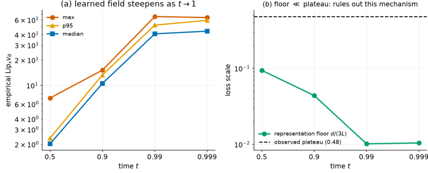
Figure 4: The empirical Lipschitz constant of \mathbf{v}_\theta blows up as t \rightarrow 1 (left); the representation floor d/(3L) is \sim 50\times below the observed loss plateau (right), ruling out this particular Lipschitz-capacity explanation and pointing toward an optimisation-limited plateau instead.
