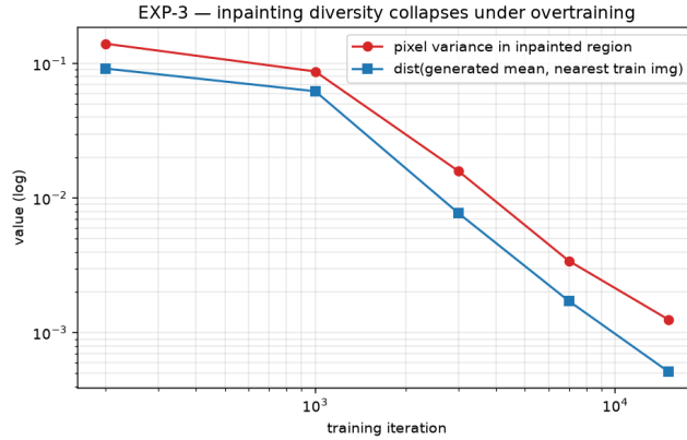
Figure 16: EXP-3 (MNIST inpainting), quantitative collapse, shown for seed 0 (whose checkpoint schedule is the finest of the three; the 3-seed statistics at the shared 15000-iteration checkpoint are in the text). The inpaint-region pixel variance and the distance to the nearest training image both fall by roughly two orders of magnitude as the loss descends.
