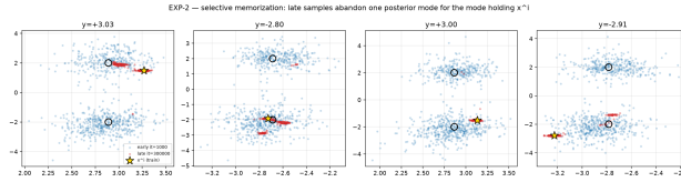
Figure 10: EXP-2 qualitative collapse. Generated samples concentrate on the posterior mode containing the memorised x^i and abandon the other, even though the analytic posterior for this observation is bimodal.
