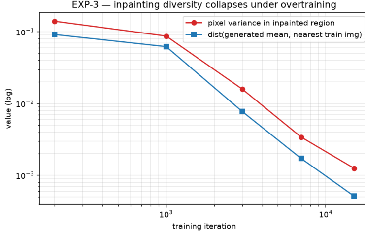
Figure 9: EXP-3 (MNIST inpainting), quantitative collapse: the inpaint-region pixel variance and the distance to the nearest training image both fall by orders of magnitude as the loss descends, while the observed-region reconstruction stays exact.
