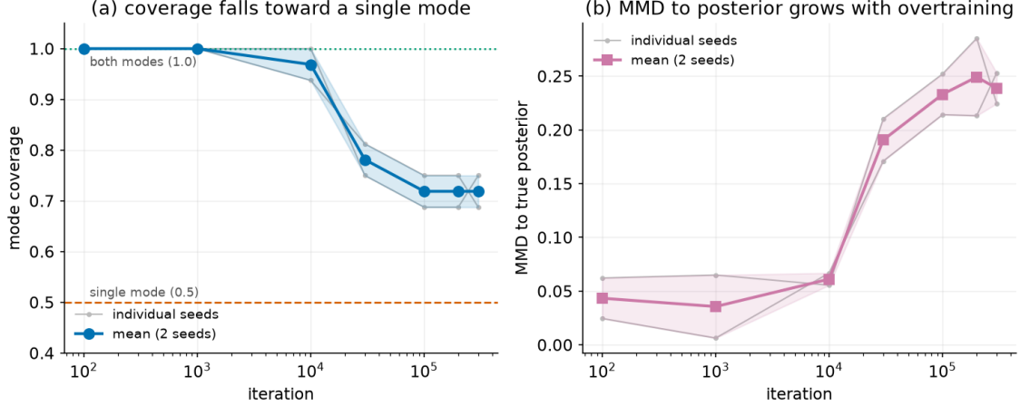
Figure 8: EXP-2 (GMM), mean of 2 seeds with per-seed traces and a \pm std band. (a) Mode coverage holds at 1.0 (both posterior modes) until \sim 10^4 iterations, then falls toward the single-mode line 0.5. (b) The MMD to the true bimodal posterior is near zero in the calibrated phase and grows as overtraining concentrates the samples on one mode. Onset matches EXP-1.
