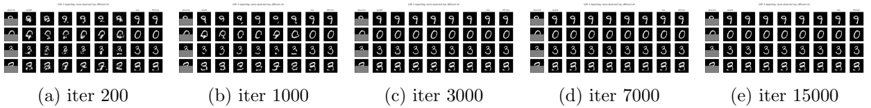
Figure 11: EXP-3 collapse trajectory (MNIST inpainting). Each grid shows completions of a fixed masked digit from different source samples x_0 . Early in training (iter 200) the completions are diverse—a calibrated conditional sampler; as the loss descends they sharpen progressively (iter 1000–7000) and, by iter 15000, are identical to one another and equal to the nearest training image (inpaint-region pixel variance 0.140 \rightarrow 0.0013 , a \sim 100\times drop). This is the same loss \rightarrow 0 -paced collapse as EXP-1, on real image data.
