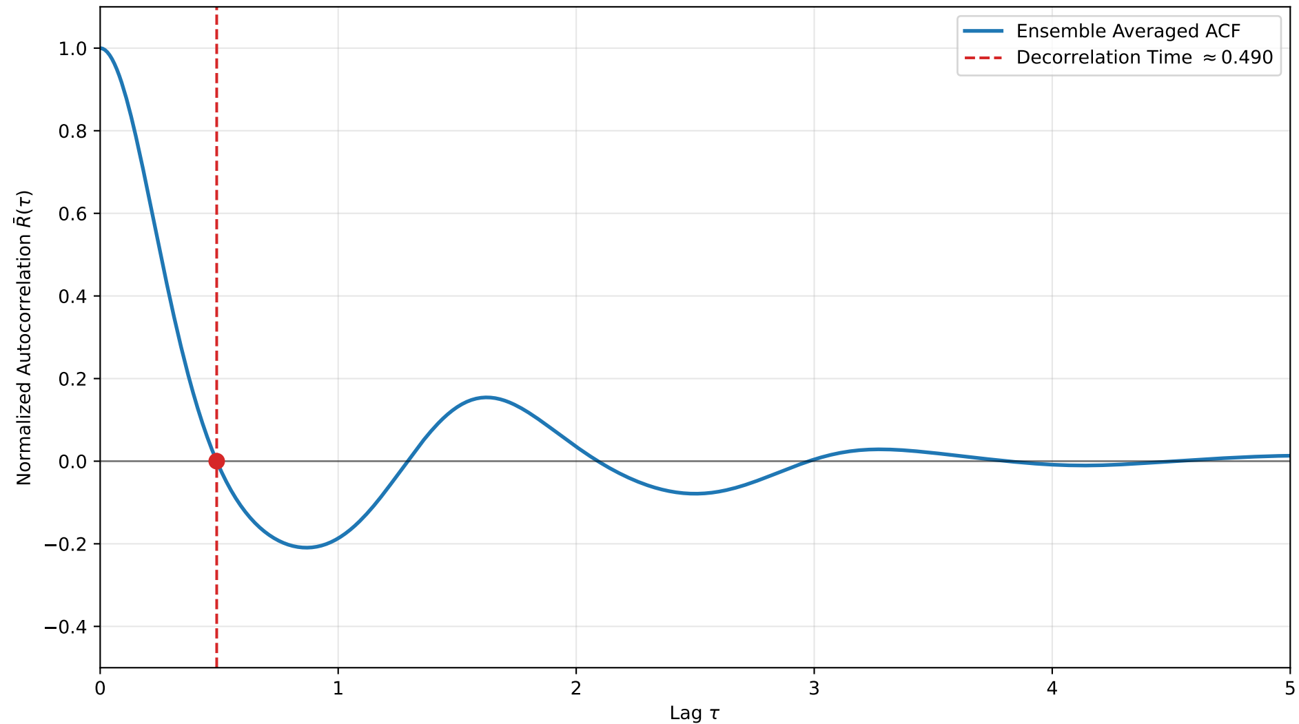
Autocorrelation & Decorrelation Time for Lorenz '96 ( j = 40, F = 7.0 )
