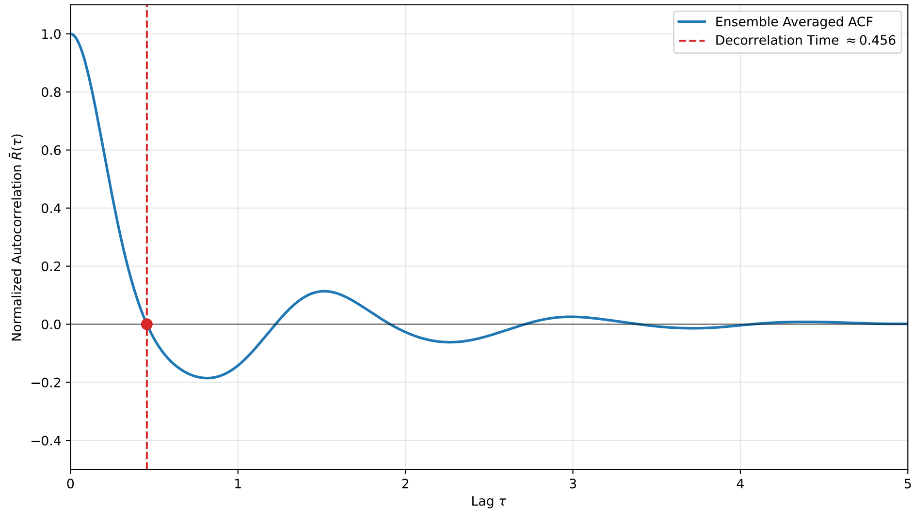
Autocorrelation & Decorrelation Time for Lorenz '96 ( j = 40, F = 8.0 )
