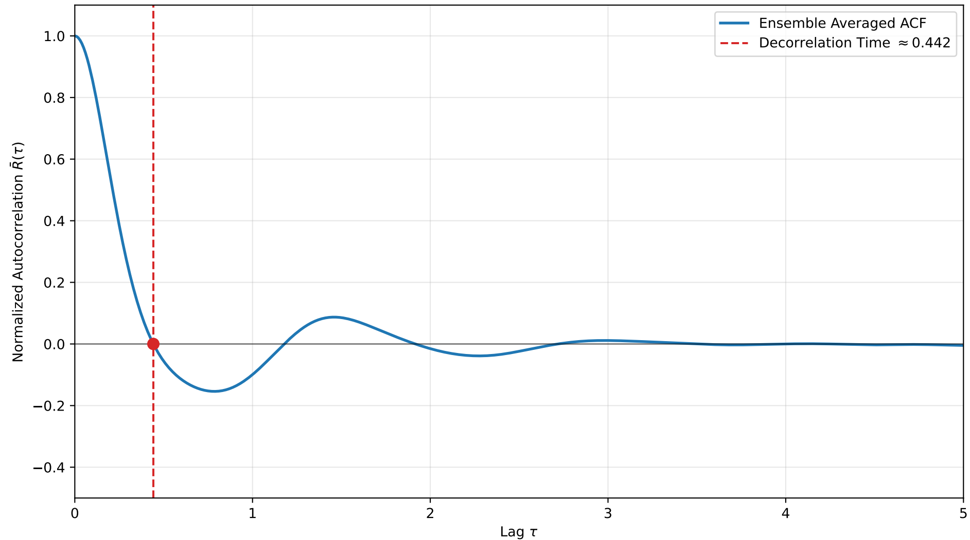
Autocorrelation & Decorrelation Time for Lorenz '96 ( j = 40, F = 9.0 )
