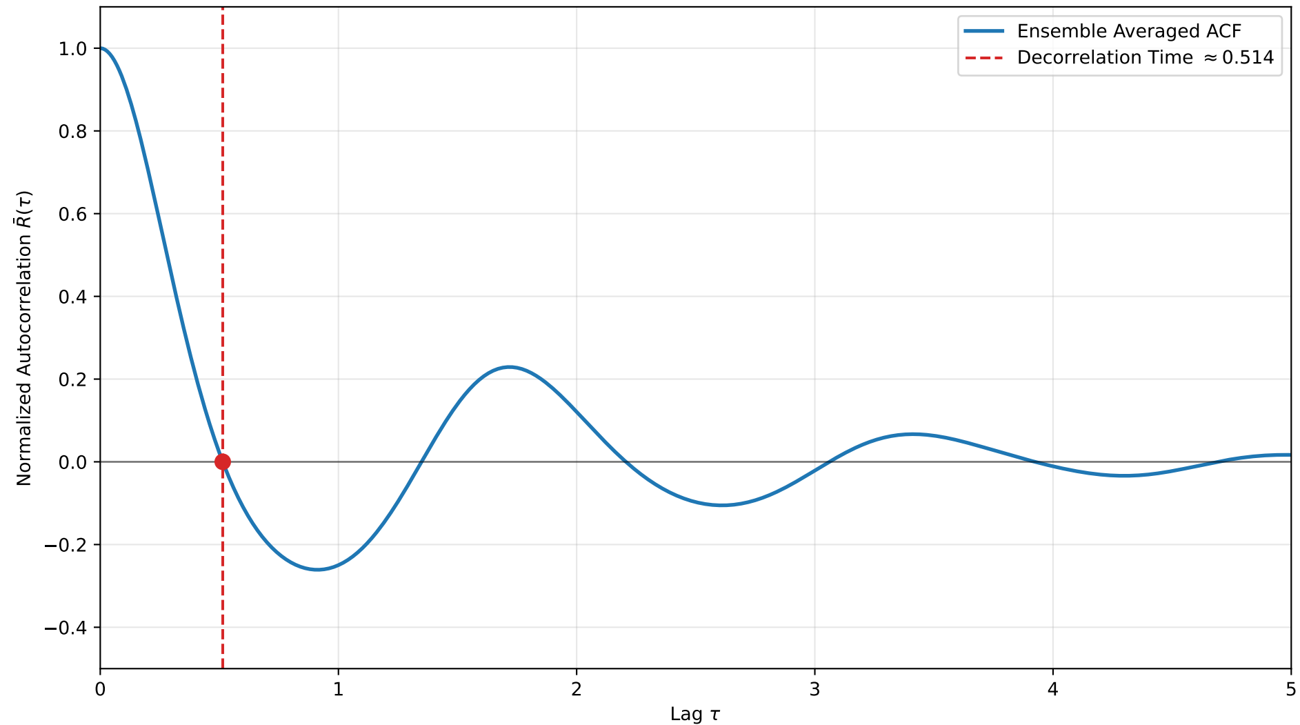
Autocorrelation & Decorrelation Time for Lorenz '96 ( j = 40, F = 6.0 )
