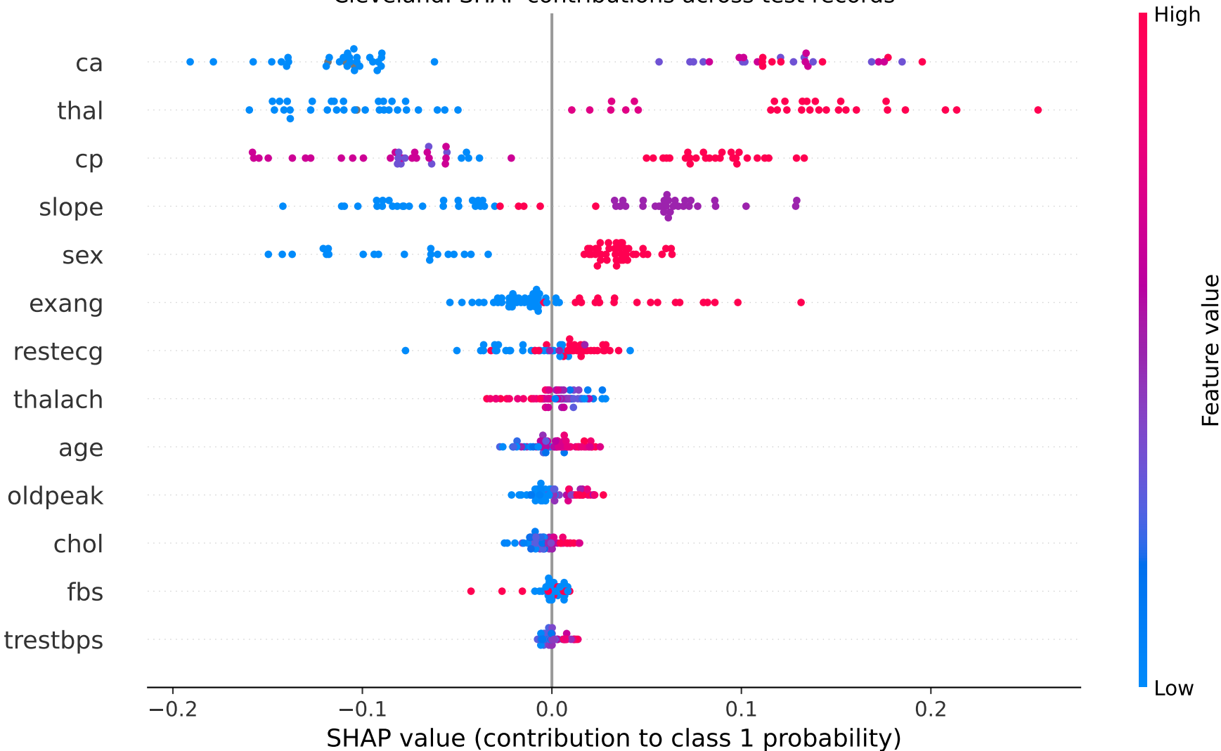
Cleveland: SHAP contributions across test records
