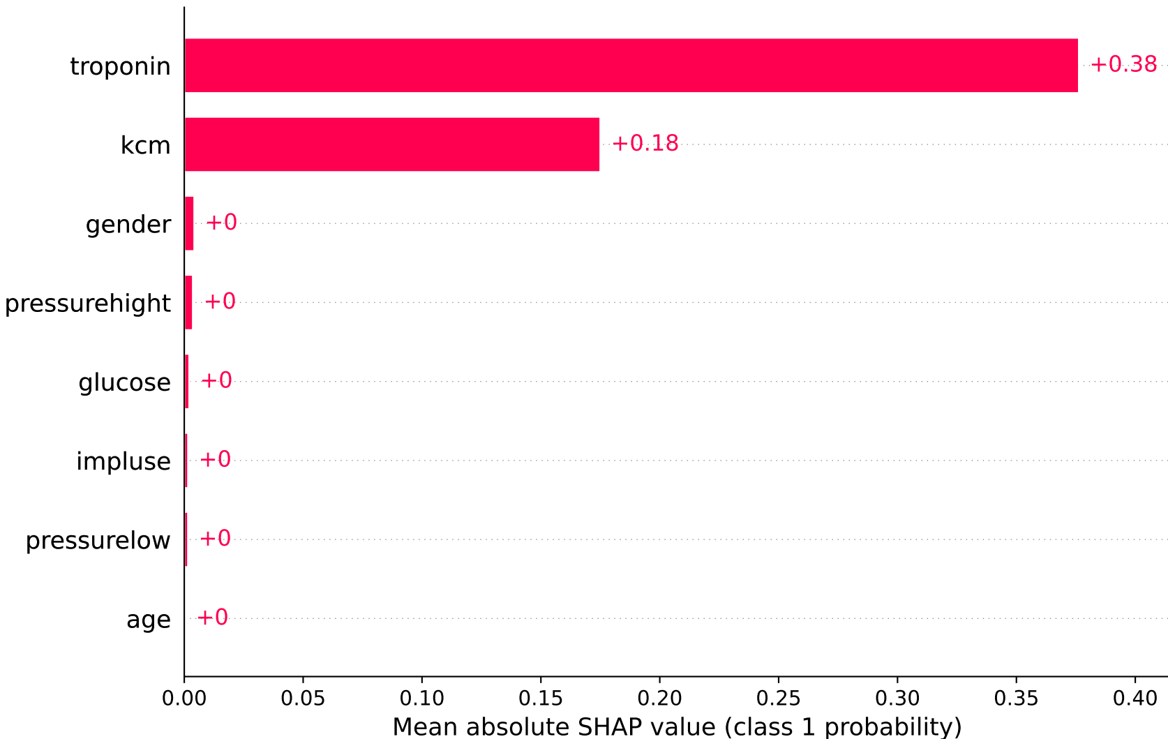
HDC: mean absolute SHAP contributions
