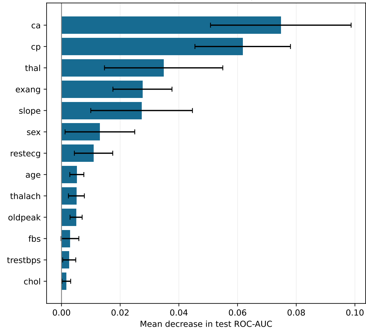
Cleveland: permutation importance
