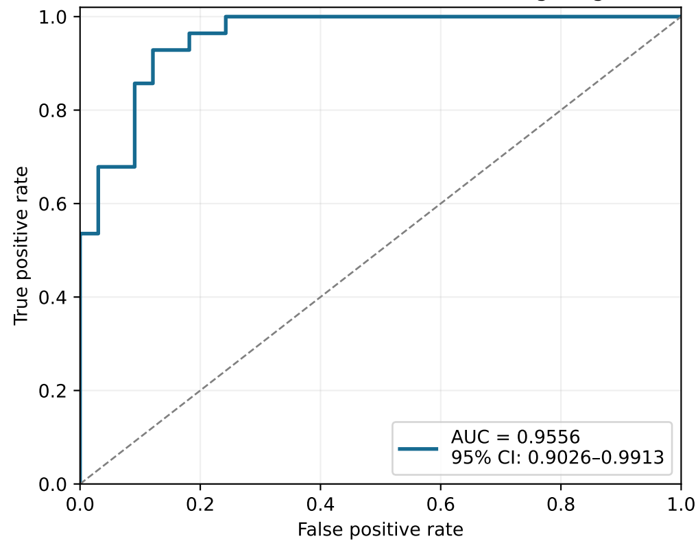
Cleveland: Extra Trees + Class weighting
