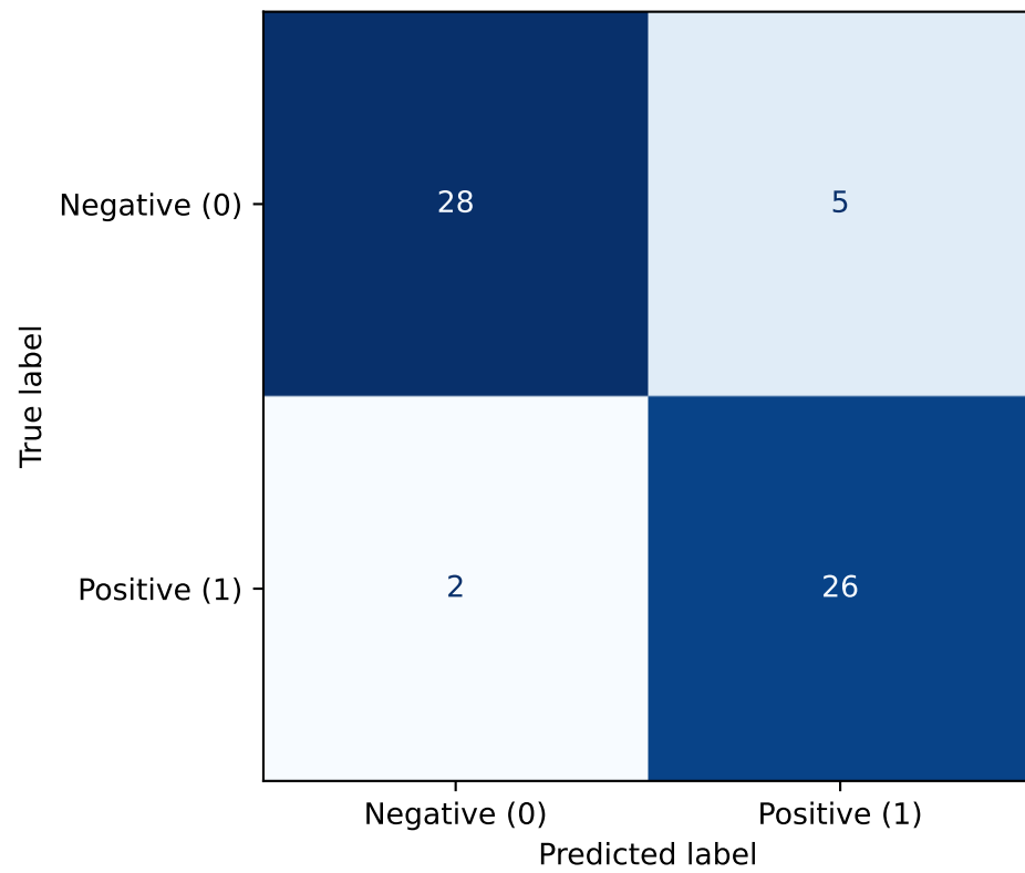
Cleveland: threshold = 0.50
