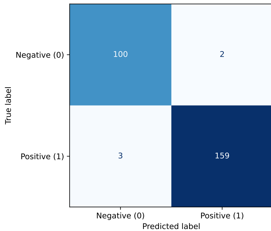
Cleveland: threshold = 0.50
