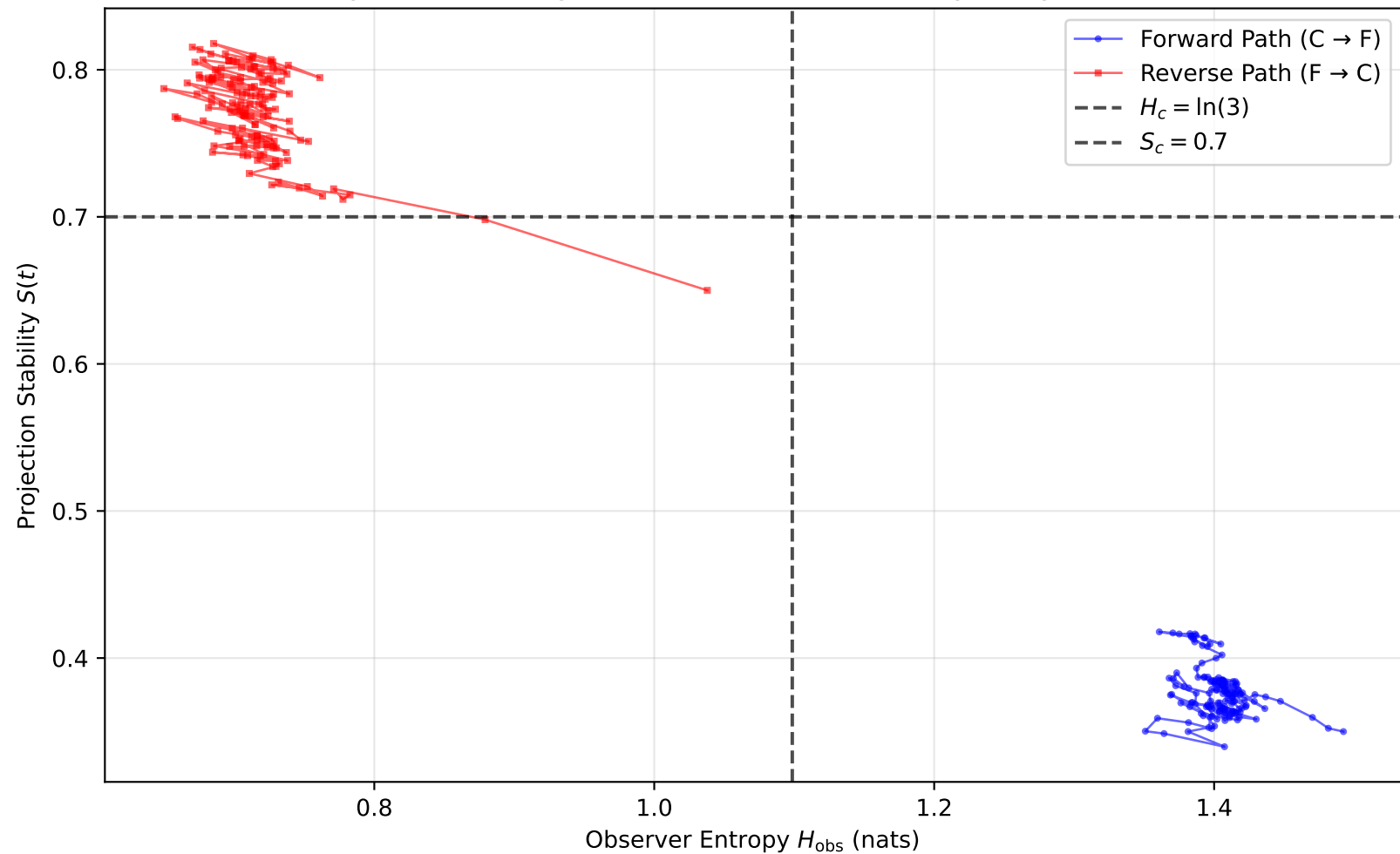
Hysteresis in Cognitive Phase Transitions (Physically Correct)
