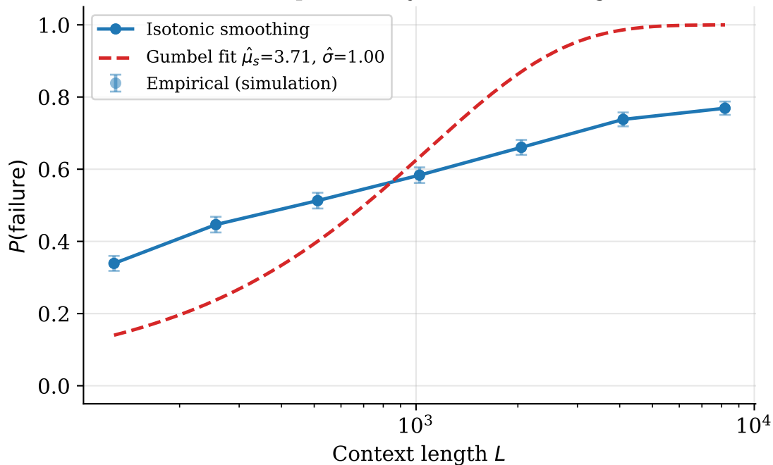
Failure probability vs. context length
