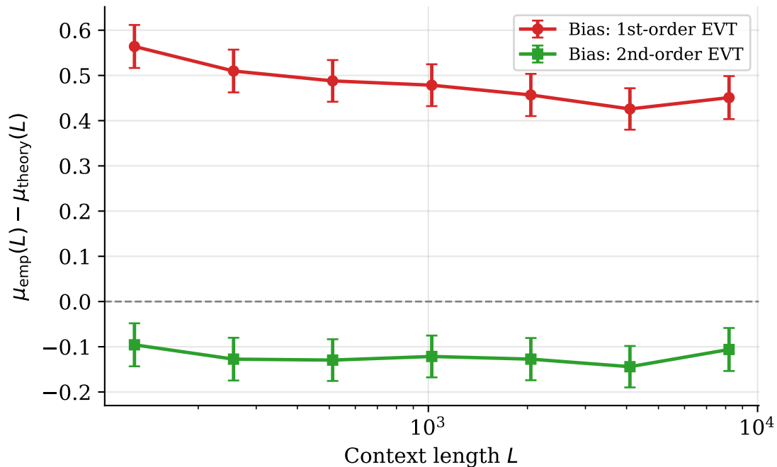
Finite-size bias: 1st vs 2nd order EVT
