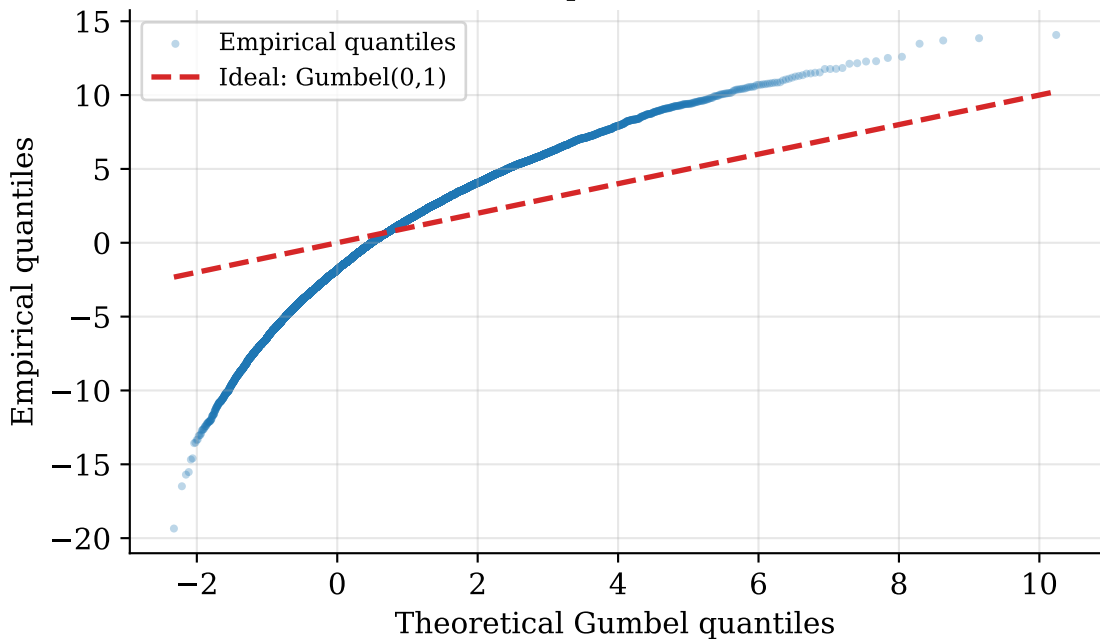
QQ-plot vs Gumbel(0,1) KS stat=0.3938, p=0.0000 (simulation)
