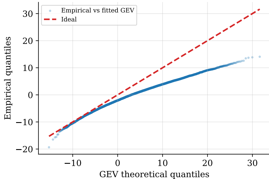
QQ vs fitted GEV \xi = -0.138 [-0.296, -0.126]
