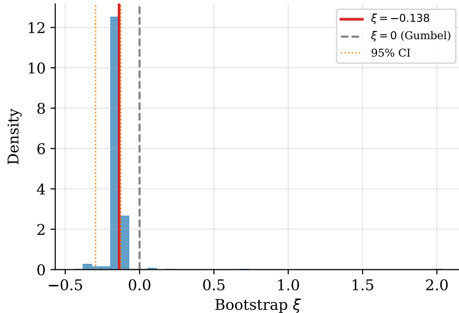
Bootstrap CI for GEV shape \xi (simulation)
