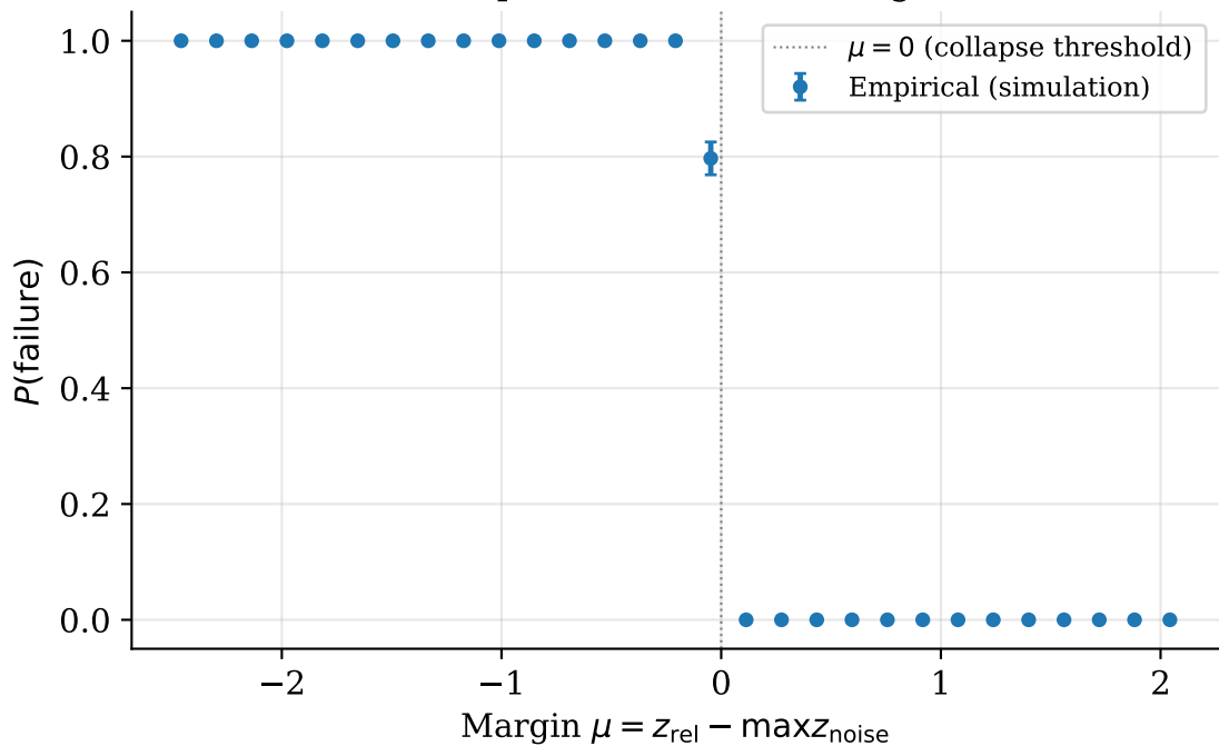
Collapse transition vs. margin
