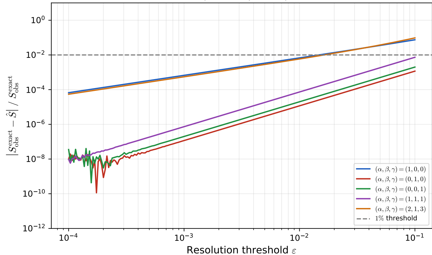
Relative error of quadratic approximation [Example 2: 5-point space]
