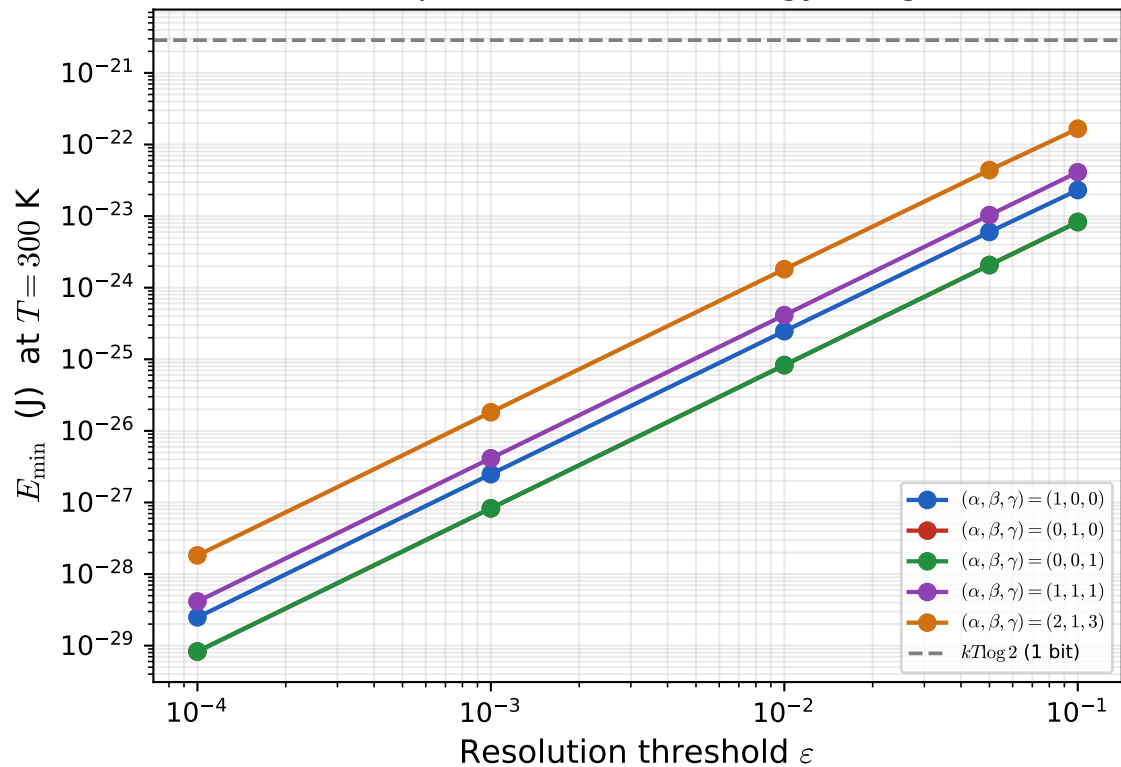
Example 2: Landauer energy budget
