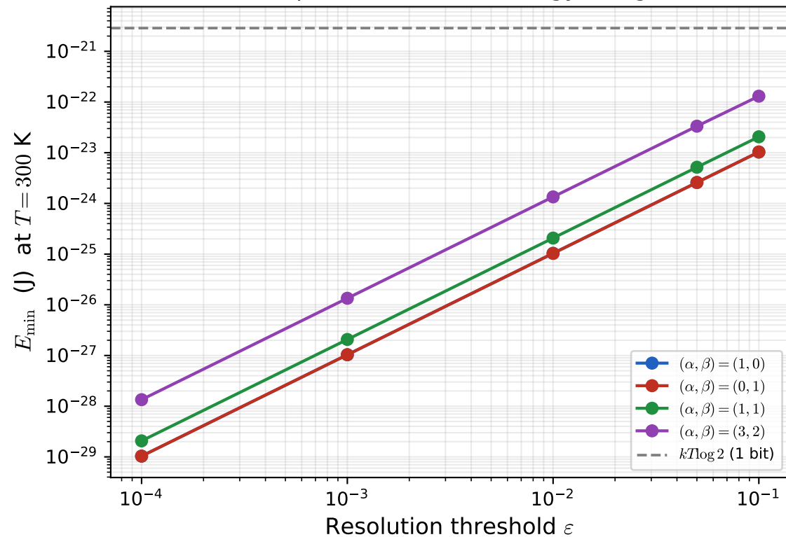
Example 1: Landauer energy budget
