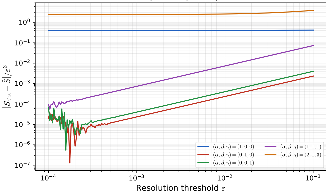
(b) Normalised remainder — confirms O(\varepsilon^3) [Example 2: 5-point space]
