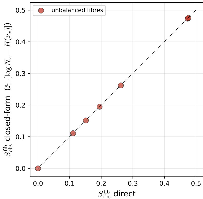
Theorem 11.9 (unbalanced extension) Unbalanced fibres
