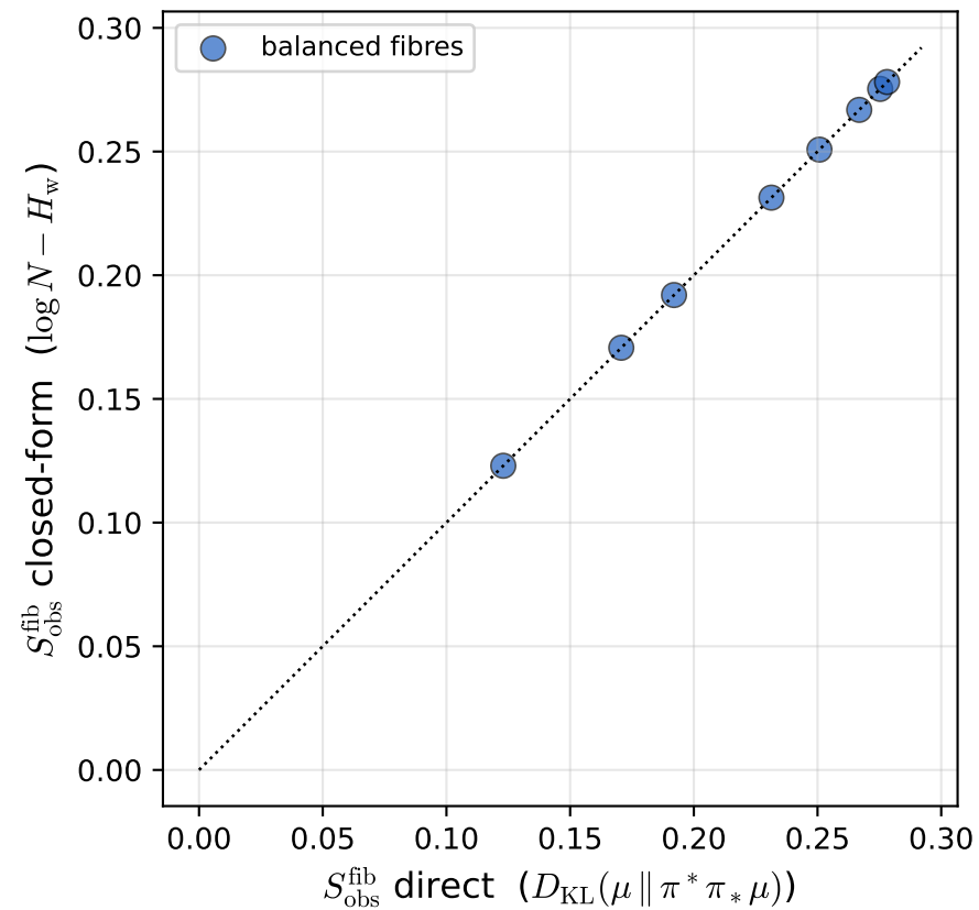
Theorem 11.9 (closed-form identity) Balanced fibres
