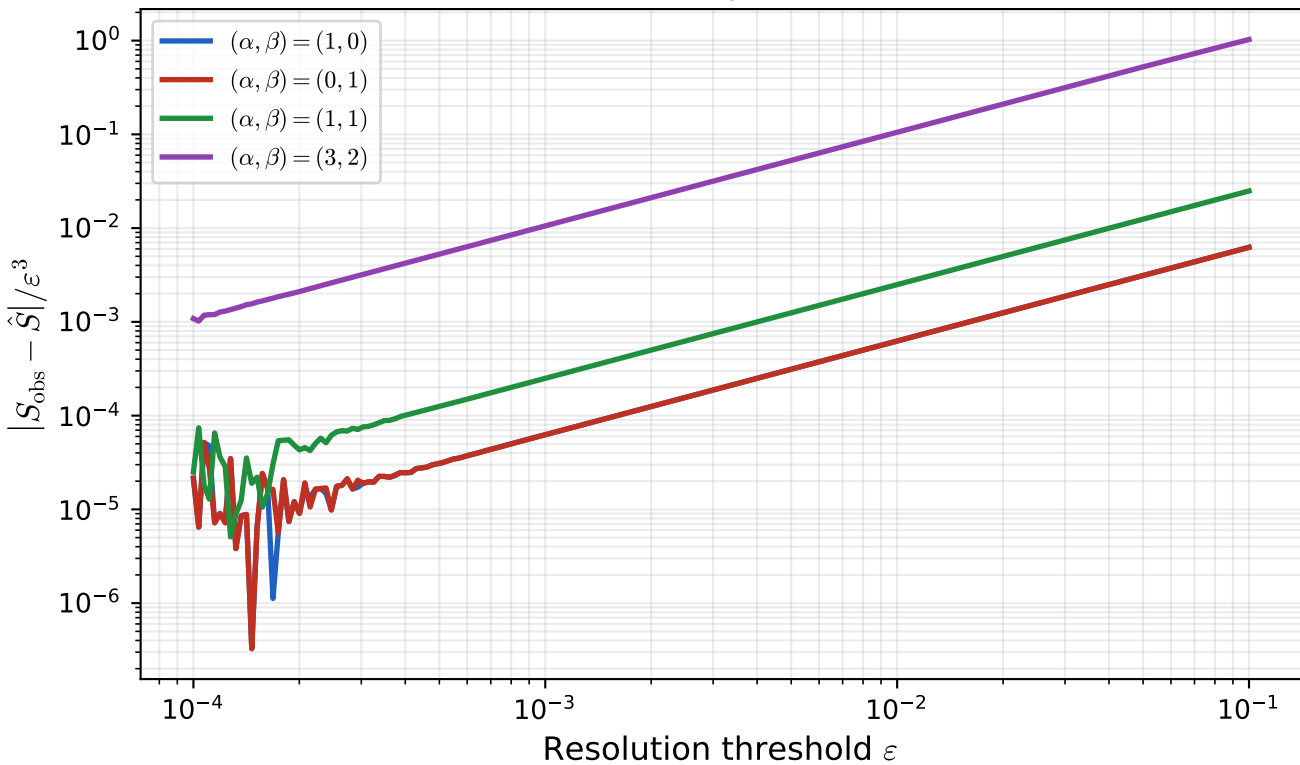
(b) Normalised remainder — confirms O(\varepsilon^3) [Example 1]
